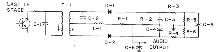
Fig. 9—Typical Ratio Detector Circuit.
