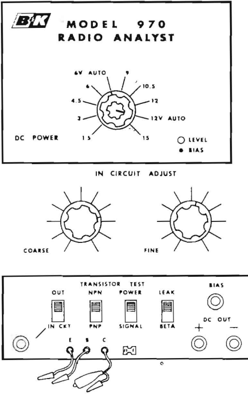
Fig. 2—Power Supply Section, Front Panel.
