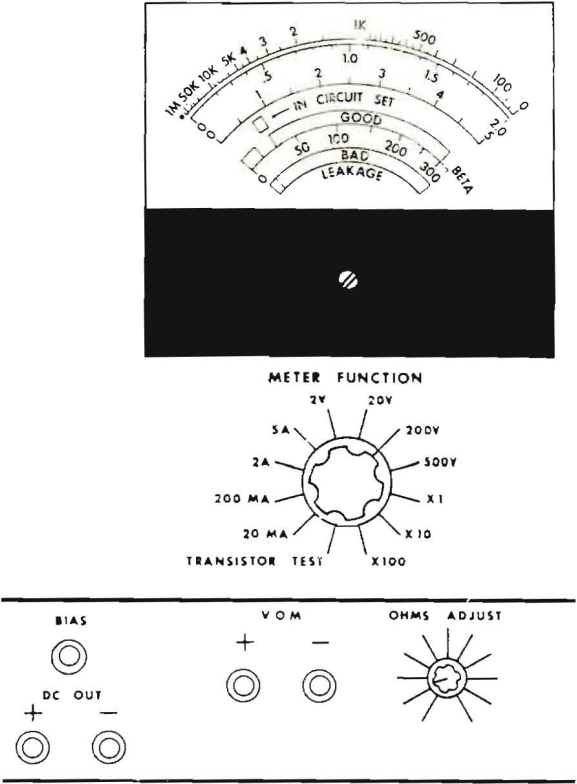
Fig. 3—VOM Section, Front Panel.
