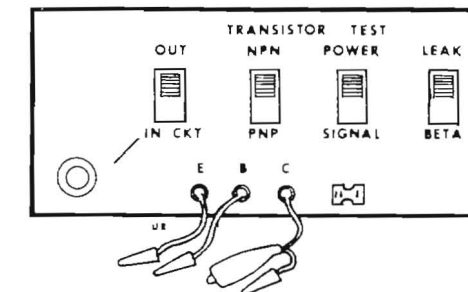
Fig. 6—Transistor Testing, Front Panel.
