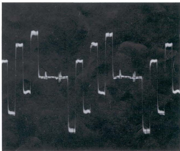
Fig. 27. Correct (B-Y) signal (blue-colour difference signal)
