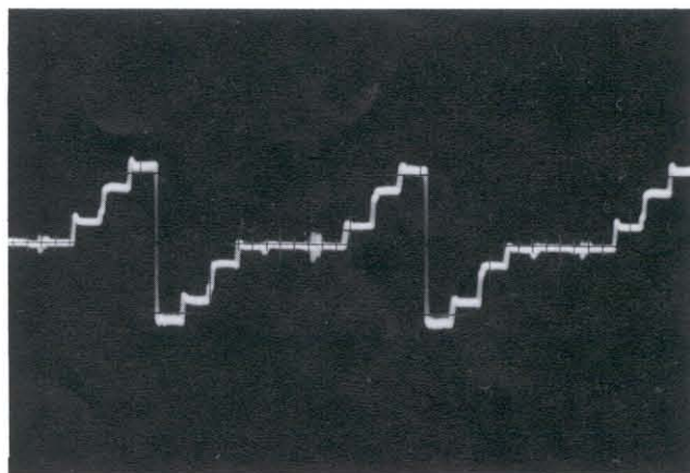
Fig. 31. Correct (G-Y) signal (green-colour difference signal)
