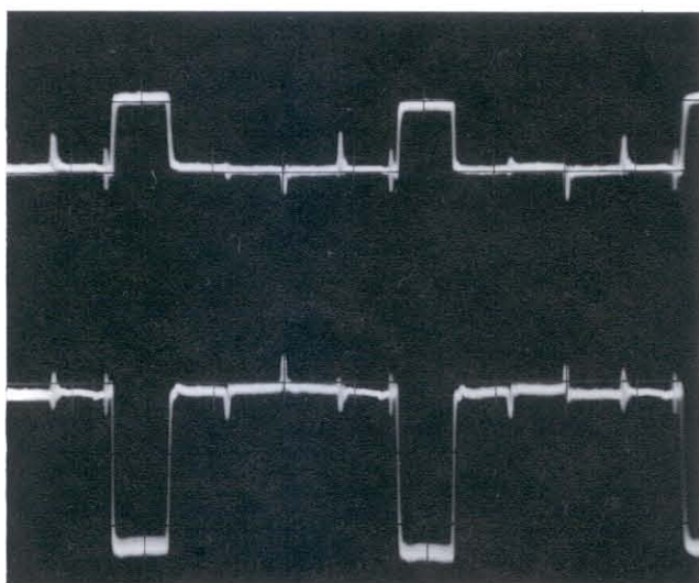
Fig. 34. Delay line and demodulators, correctly adjusted
