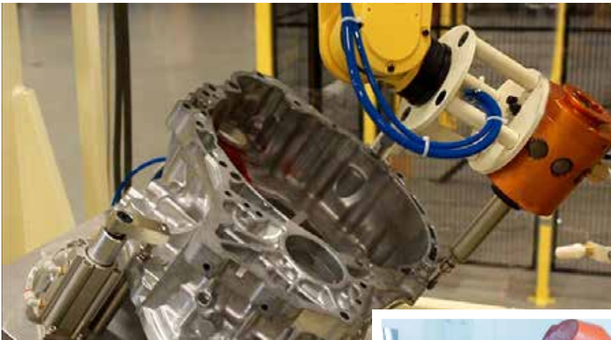
ROBOTIC DEBURRING
