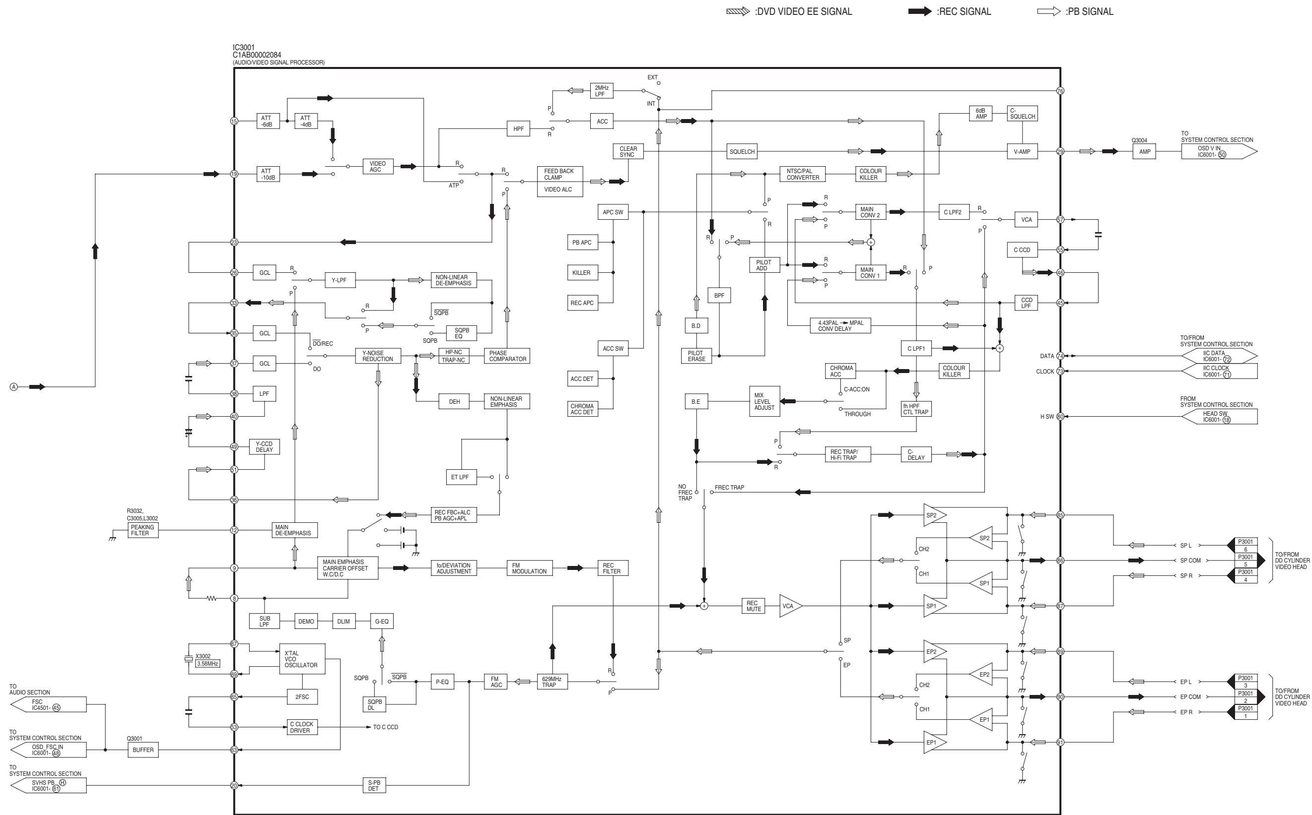
DMR-ES35VEE/GCS/GN/GC Analog Video Block Diagram 2/2
