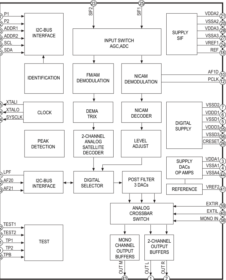
IC7301(NICAM/A2) NICAM DECODER IC-DETAIL BLOCK DIAGRAM
