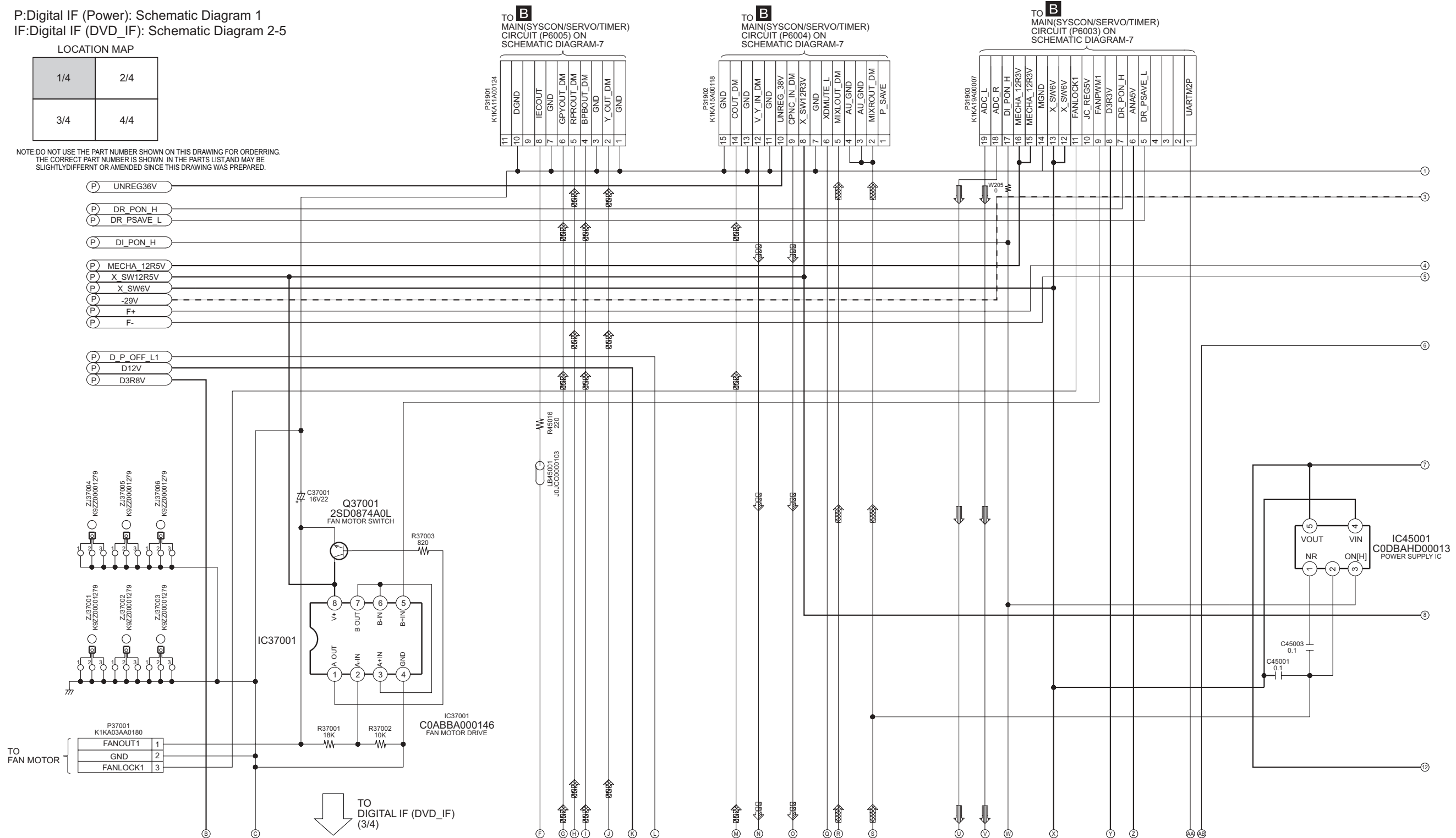
DMR-ES35VEE/GCS/GC/GN DIGITAL IF (DVD_IF) CIRCUIT
