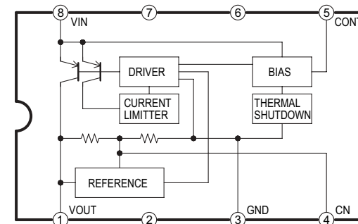
IC7402 TU +5V SWITCHING REG. IC-DETAIL BLOCK DIAGRAM
