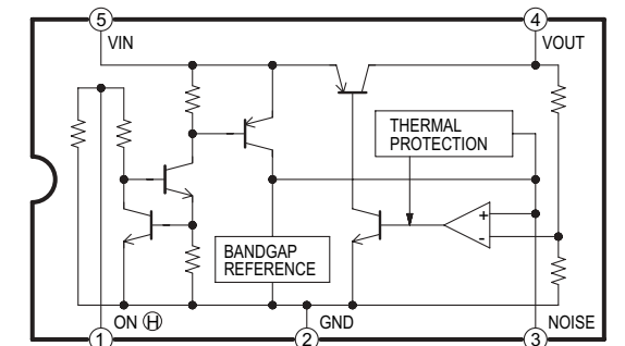
IC3701 Detail Block Diagram IC4801 Detail Block Diagram IC6001 Detail Block Diagram IC7402 Detail Block Diagram DMR-ES35VEE/GCS/GC/GN IC-Detail Block Diagram
