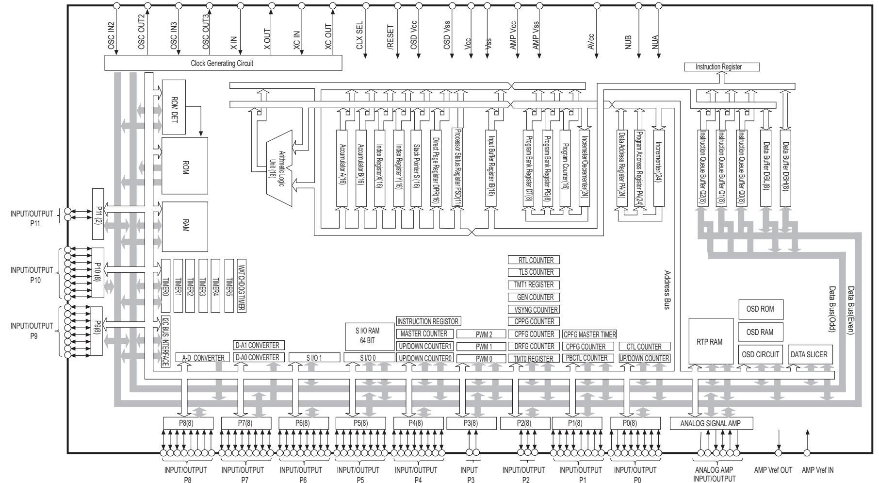
IC6001 MICRO PROCESSOR IC-DETAIL BLOCK DIAGRAM
