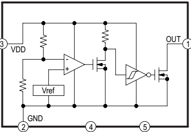
IC7502 VOLTAGE DETECTOR IC-DETAIL BLOCK DIAGRAM
