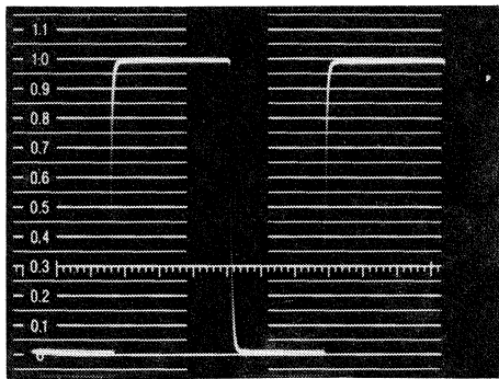
Fig. 6-1 VOLTS FULL SCALE control set to 1 V CAL.
