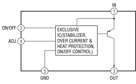
PQ2TZ15U (IC142)
