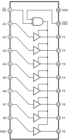
SN74LV541APWR (IC708, 709)
