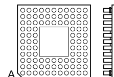
1 BOTTOM VIEW 156PIN BGA
