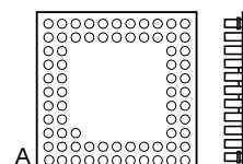
1 BOTTOM VIEW 288PIN BGA
