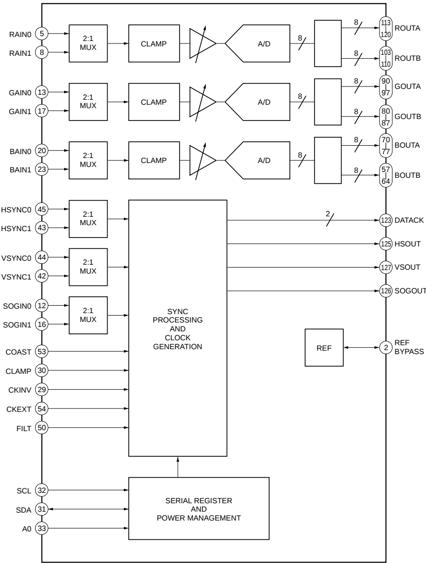
AD9888K-100 (IC403)
