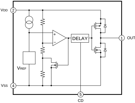
S-80928ANMP-DDR-T12 (IC405, 504, 526, 704)
