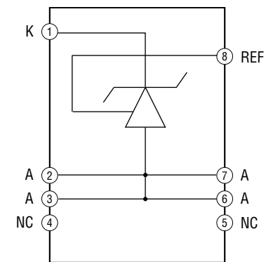
TL431BCDR2 (IC701)
