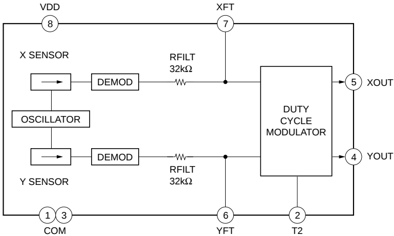
ADXL202JE-REEL (IC603)
