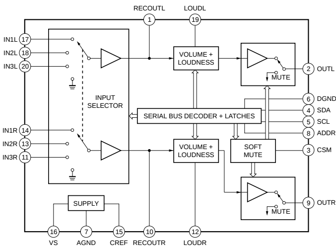
TDA7309D013TR (IC201)
