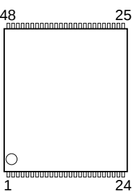
TOP VIEW 48PIN TSOP
