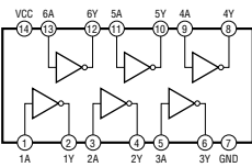
SN74LV04APWR (IC710)
