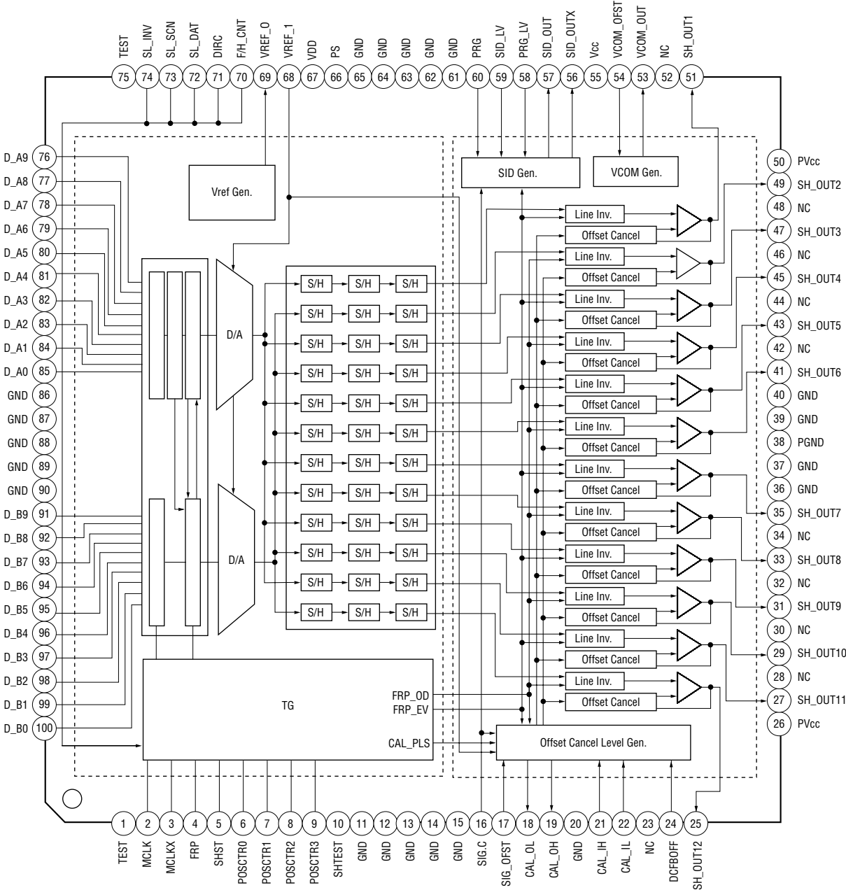
CXA3562AR-T6 (IC771, 820, 860)
