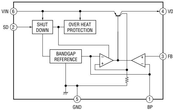
TK11900MTL (IC772)
