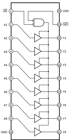
SN74LV541APWR (IC501-507)
