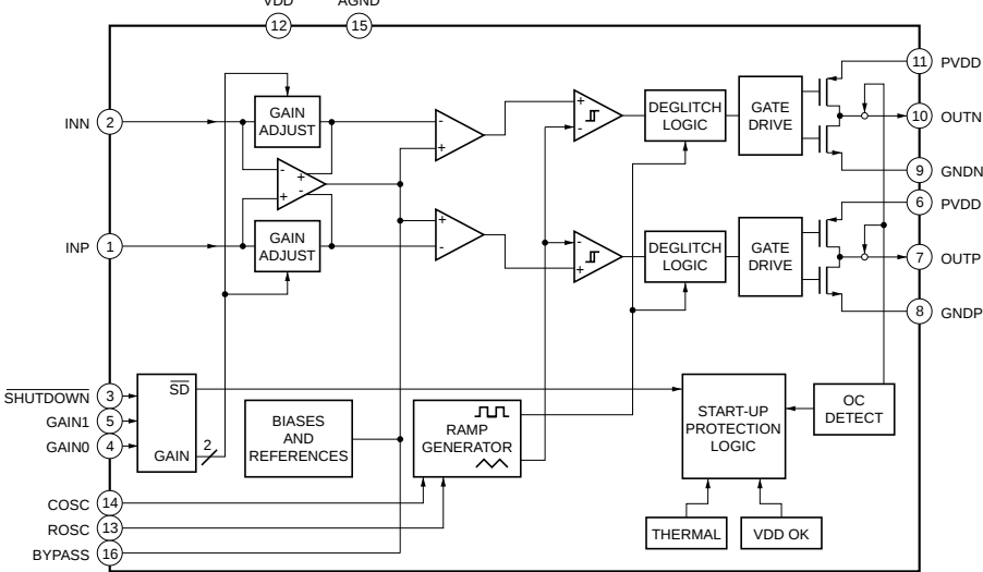
TPA2000D1PW (IC202)
