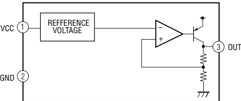
BA12FP-E2 (IC145)
