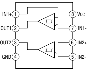
SN75157PS-EEL (IC403)
