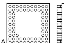
1 BOTTOM VIEW 256PIN BGA
