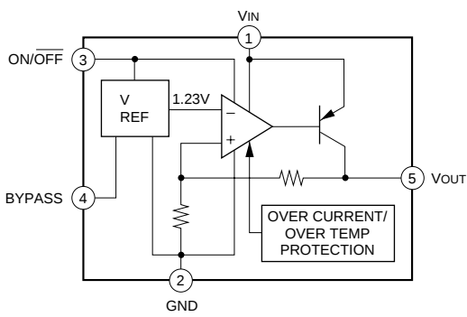
LP2985IM5X-3.3 (IC224, 402)
