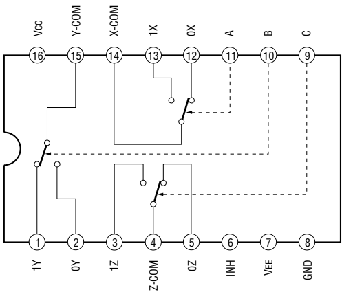
SN74LV4053APWR (IC301, 304)
