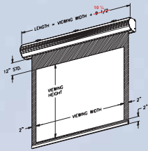
LECTRIC I MOTORIZED PROJECTION SCREEN WALL OR CEILING MOUNT
