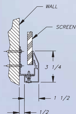
Deluxe Wide Frame with black velvet finish
