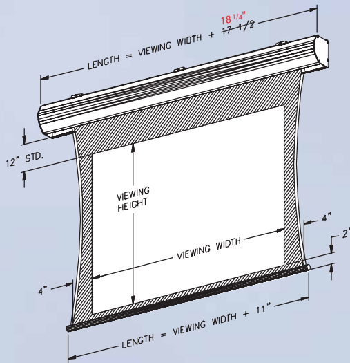
Vutec's unique wall or ceiling-mounted housing
