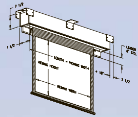
LECTRIC II MOTORIZED PROJECTION SCREEN FLUSH CEILING MOUNT
