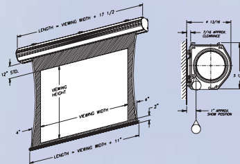
LECTRIC III MOTORIZED TAB-TENSIONED PROJECTION SCREEN WALL OR CEILING MOUNT
