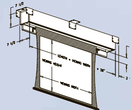
LECTRIC IV MOTORIZED TAB-TENSIONED PROJECTION FLUSH CEILING MOUNT
