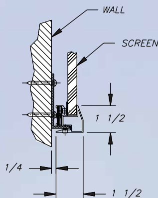
Standard Frame Flat black epoxy coated or optional black velvet finish.
