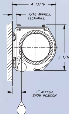
Vutec's unique wall or ceiling-mounted housing
