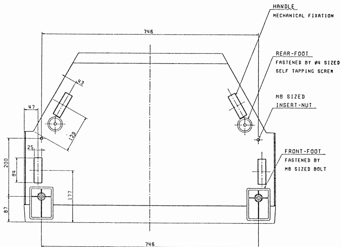
BOTTOM VIEW
