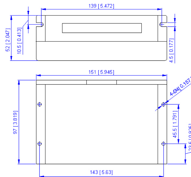
Figure 1: Mechanical specifications
