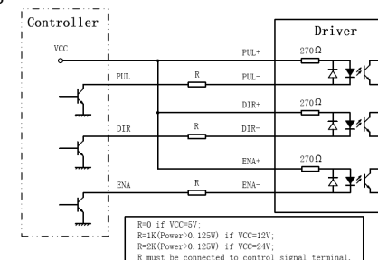
Figure 3: Connections to open-collector signal (common-anode)
