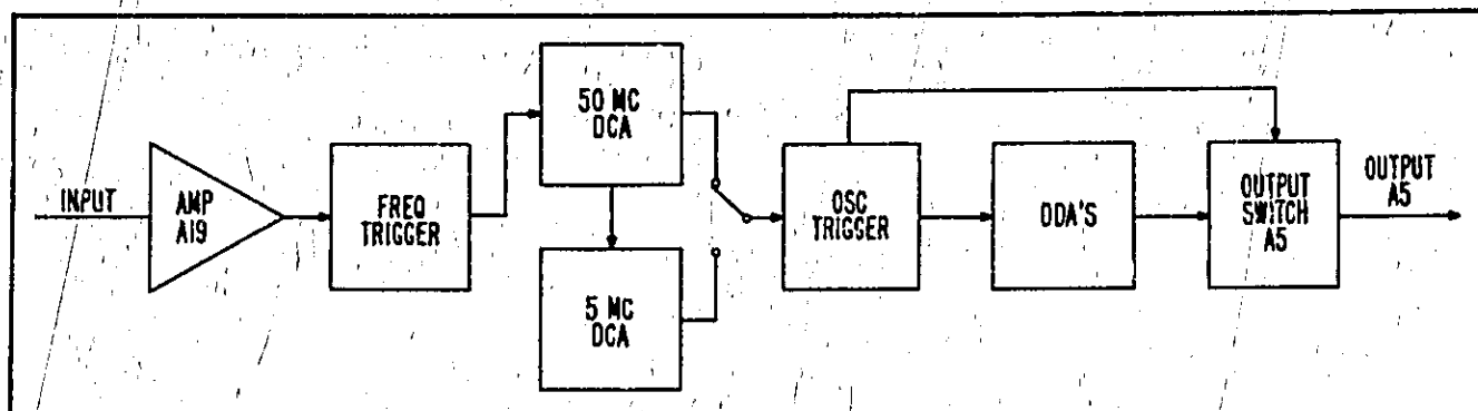
Figure 2-11. Scaler Operation
