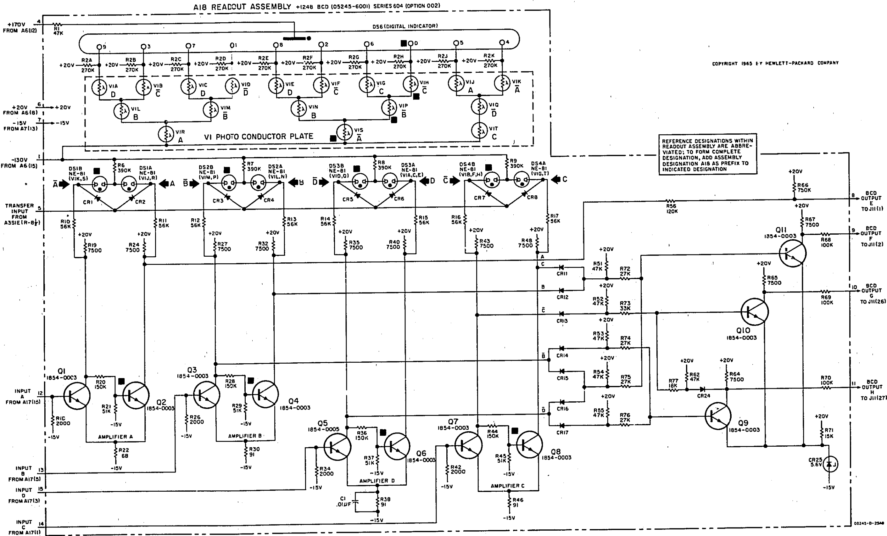
Figure 7-15. A18 Readout (05245-6001) Option 002 7-29
