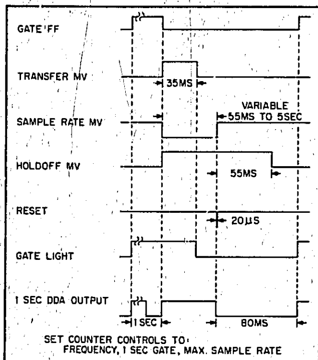
Figure 2-12. Time Sequence
