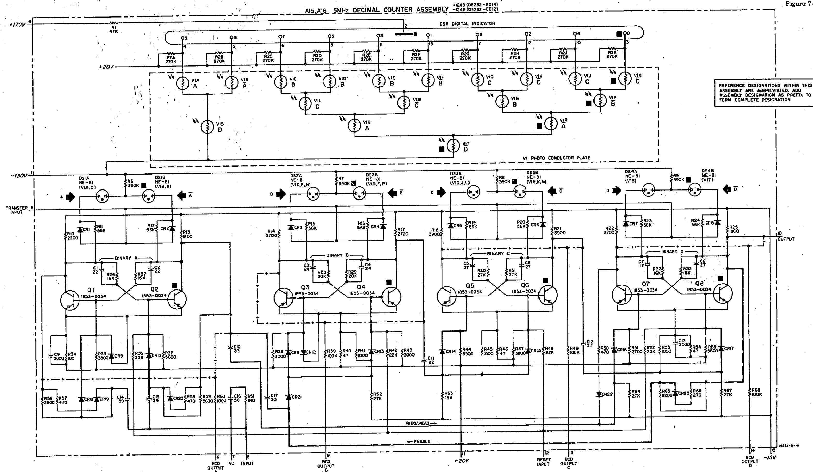
Figure 7-12. A15, A16 Decimal Counter (05232-6014, 6012) Option 002, 003
