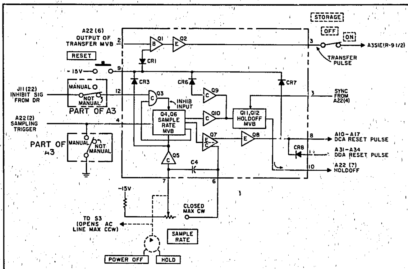
Figure 2-19. Sampling Control Block Diagram
