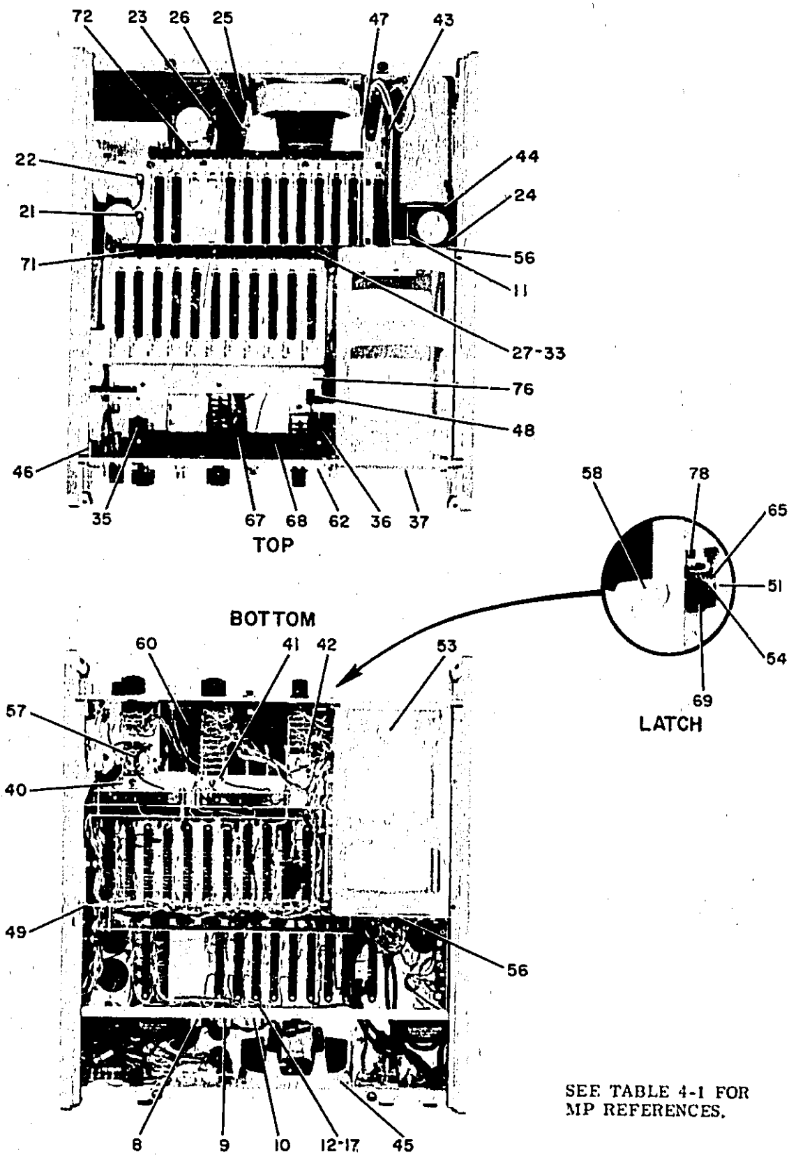
Figure 4-2. Mechanical Parts Locations
