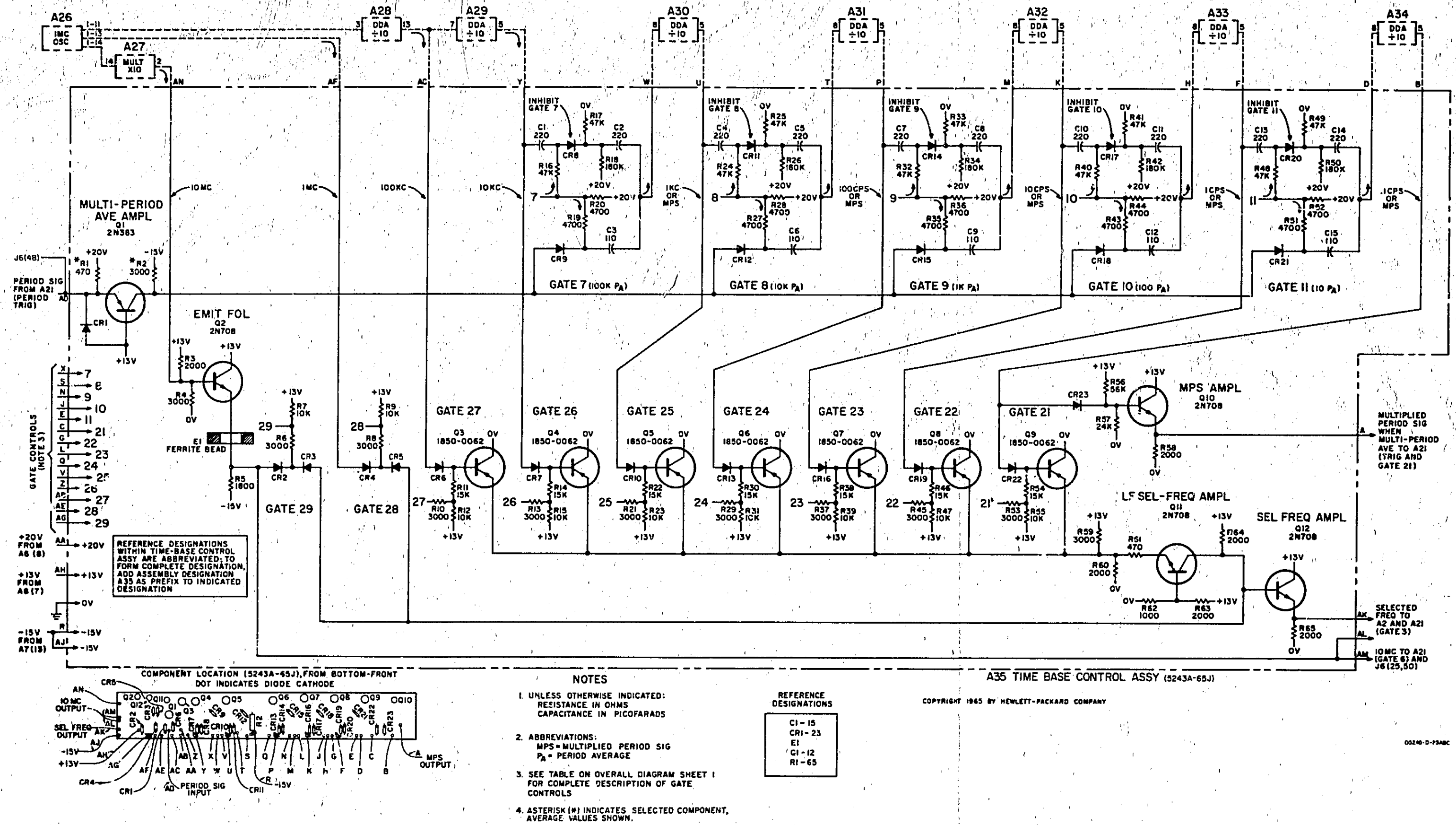
Figure 7-25. A35 Time Base Control
