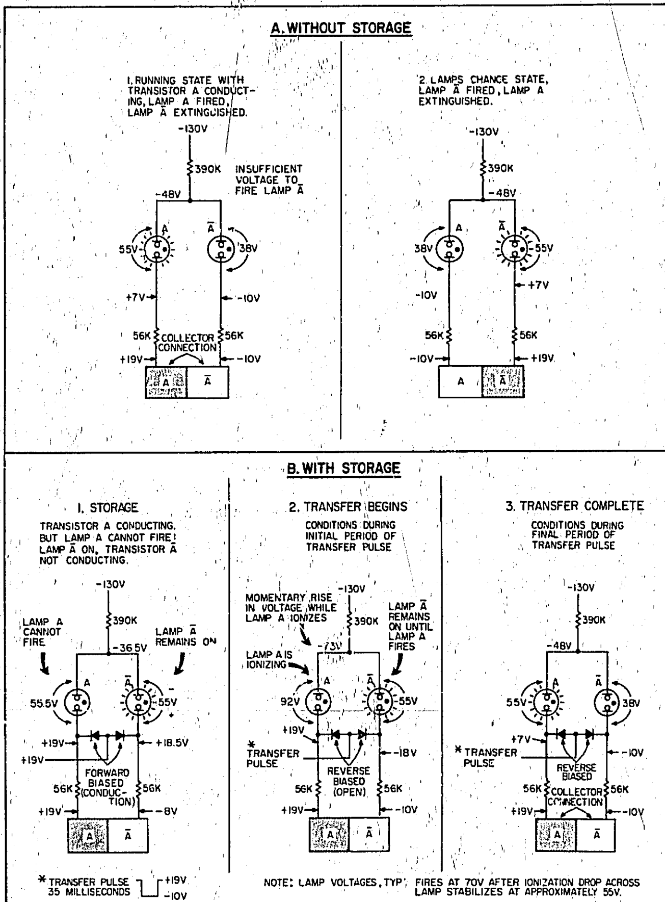
Figure 2-8. Lamp Control
