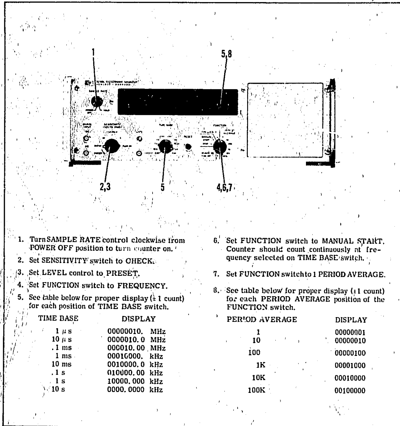
Figure 6-2. Self Check
