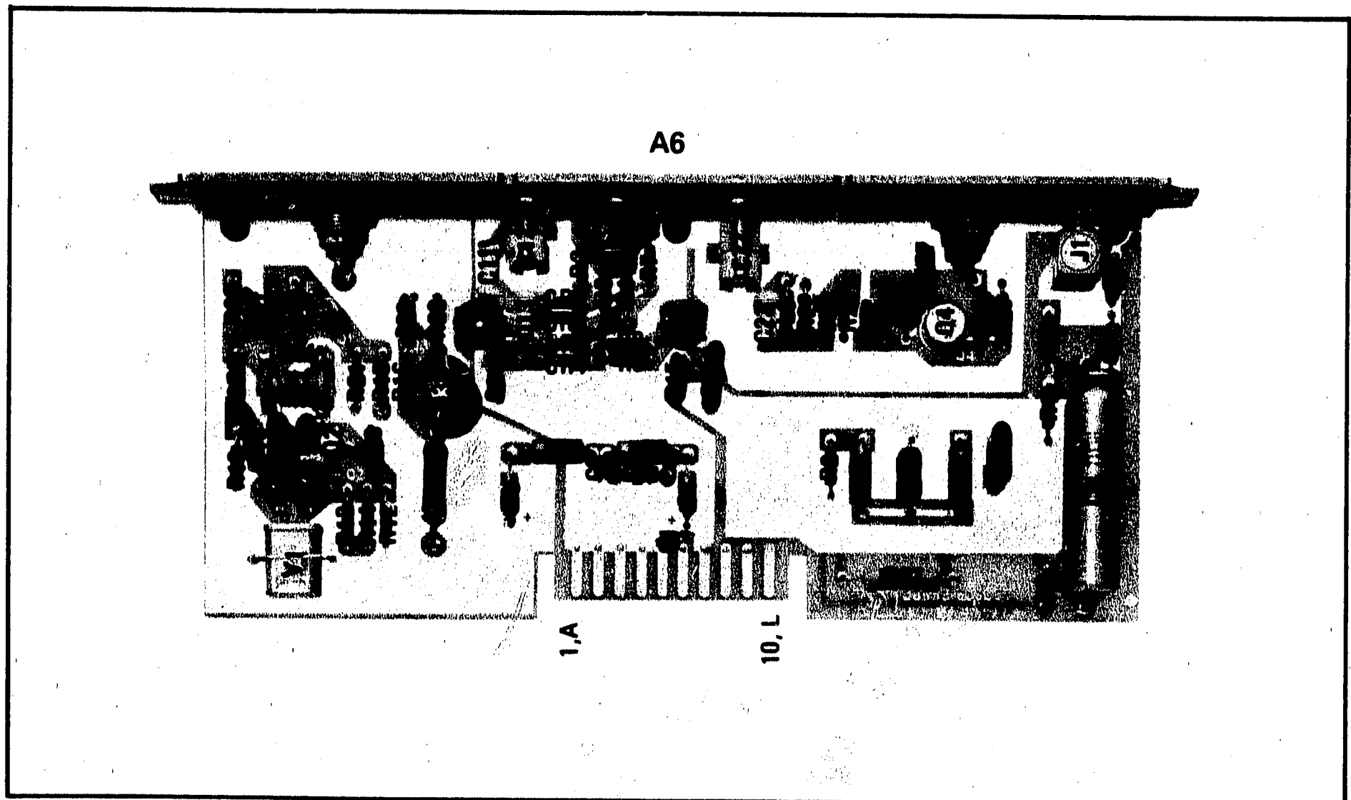
Figure 8-25. Frequency Converter Assy A6 Component Locations
