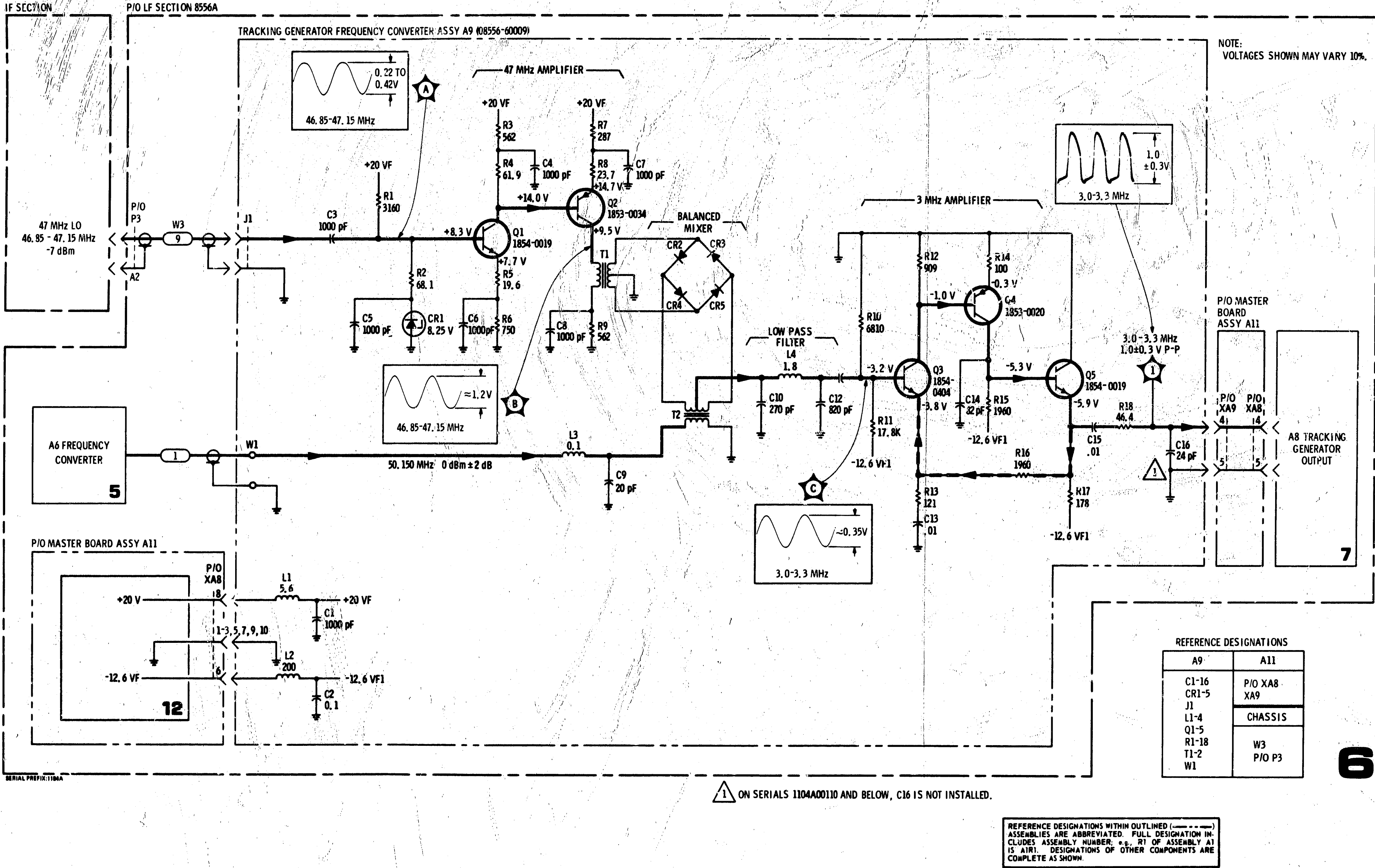
Figure 8-28. Tracking Generator Frequency Converter: A9
