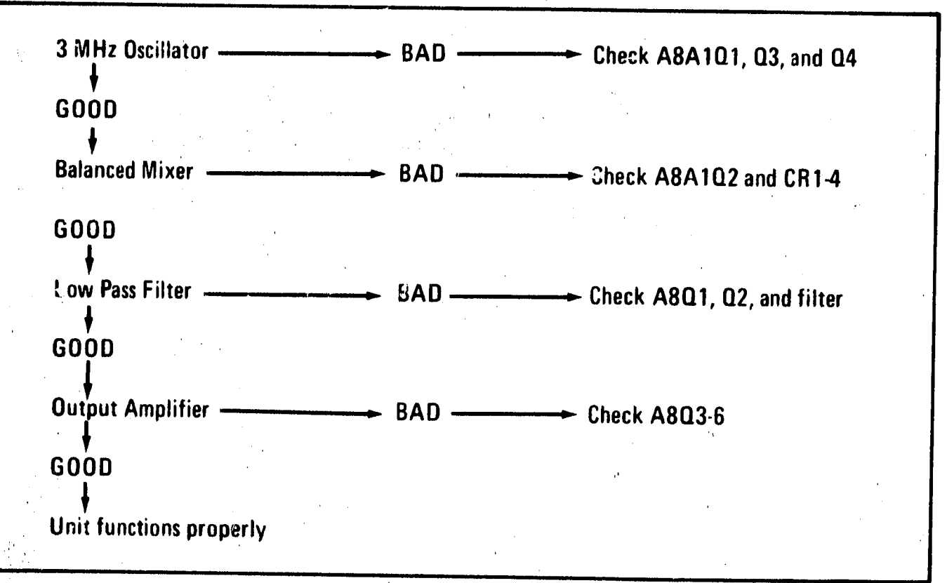
Troubleshooting Tree
