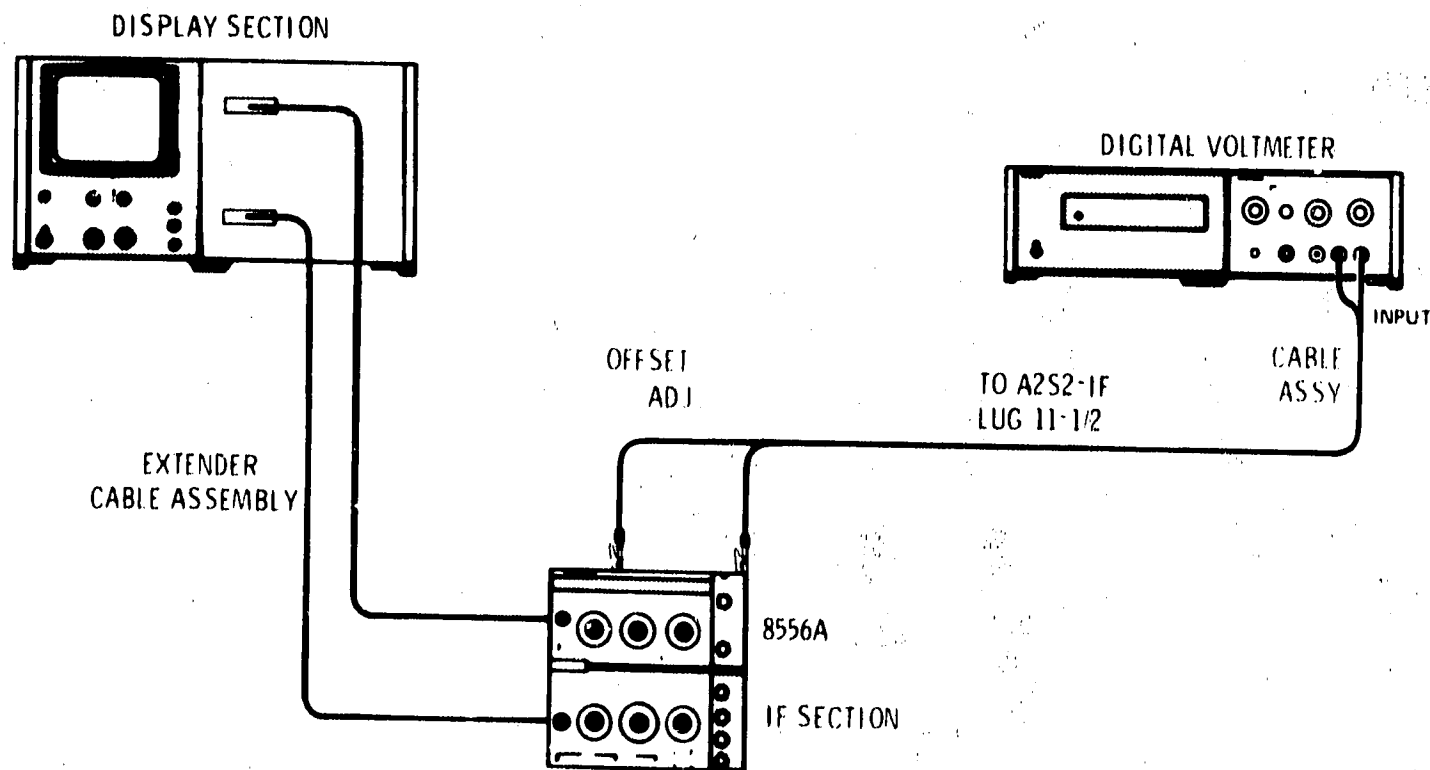
Figure 5-6. Frequency Calibration Adjustment Test Setup
