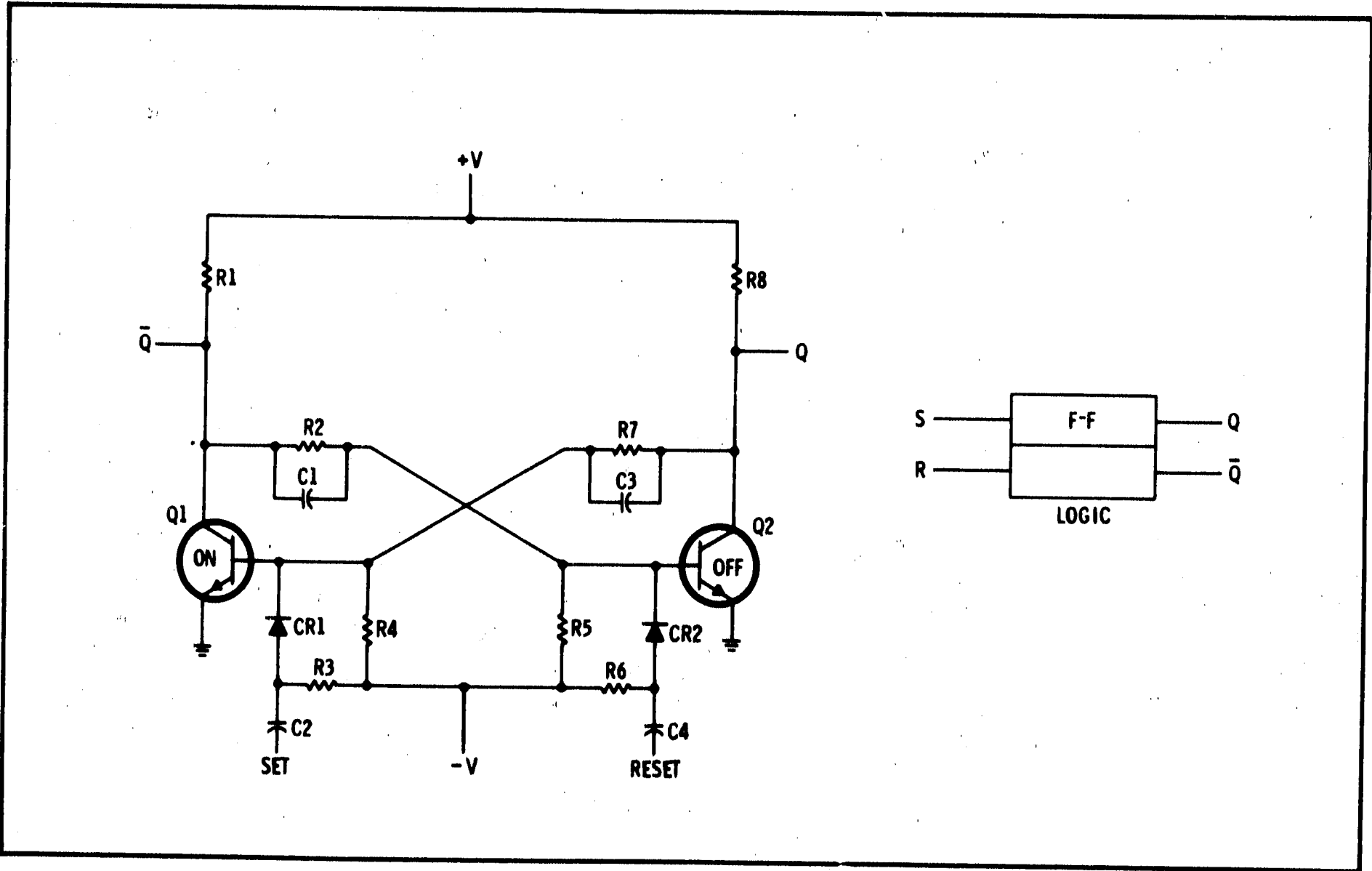
Figure 8-7. RS Flip-Flop
