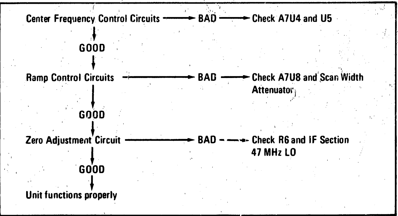
Troubleshooting Tree
