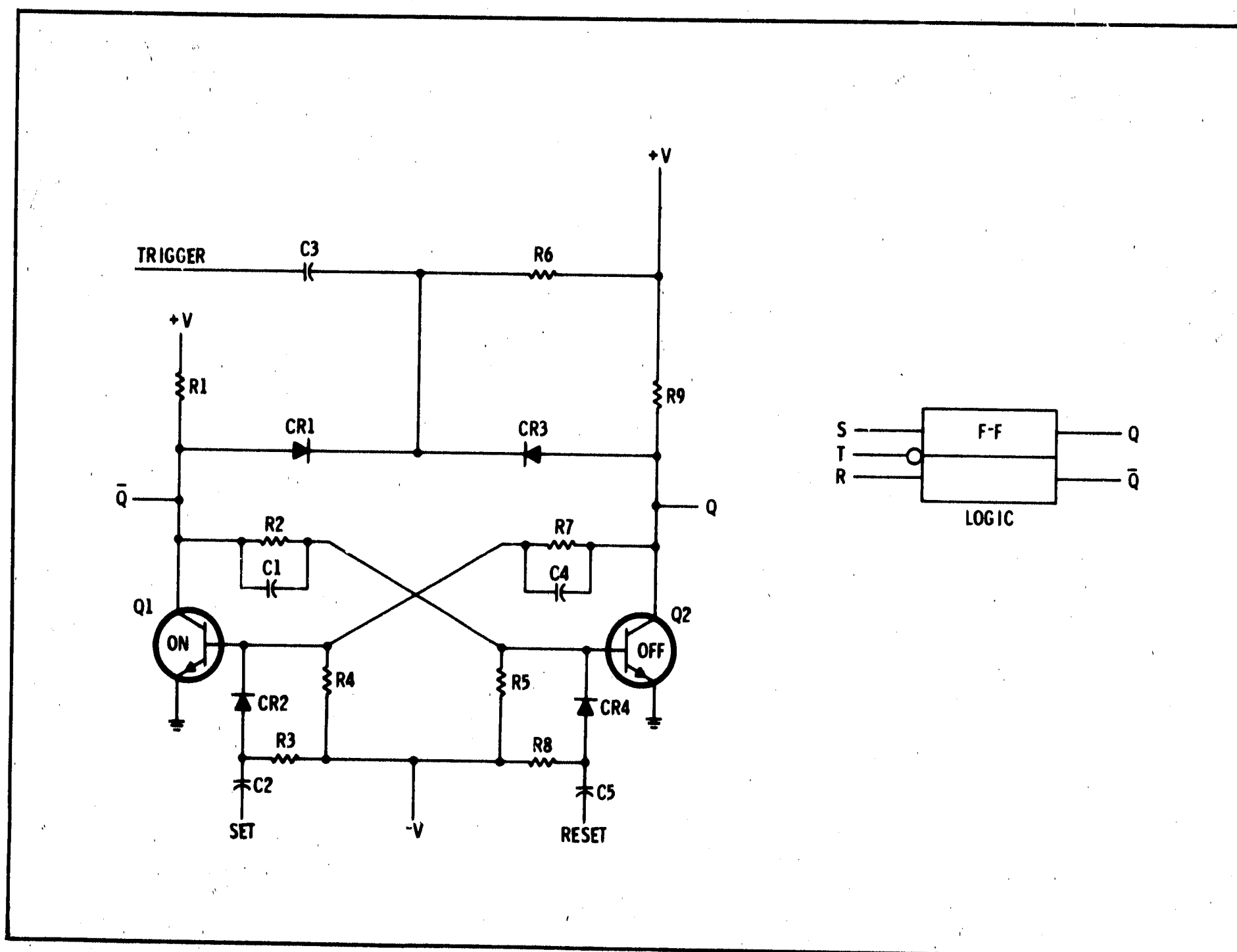
Figure 8-8. RST Flip-Flop
