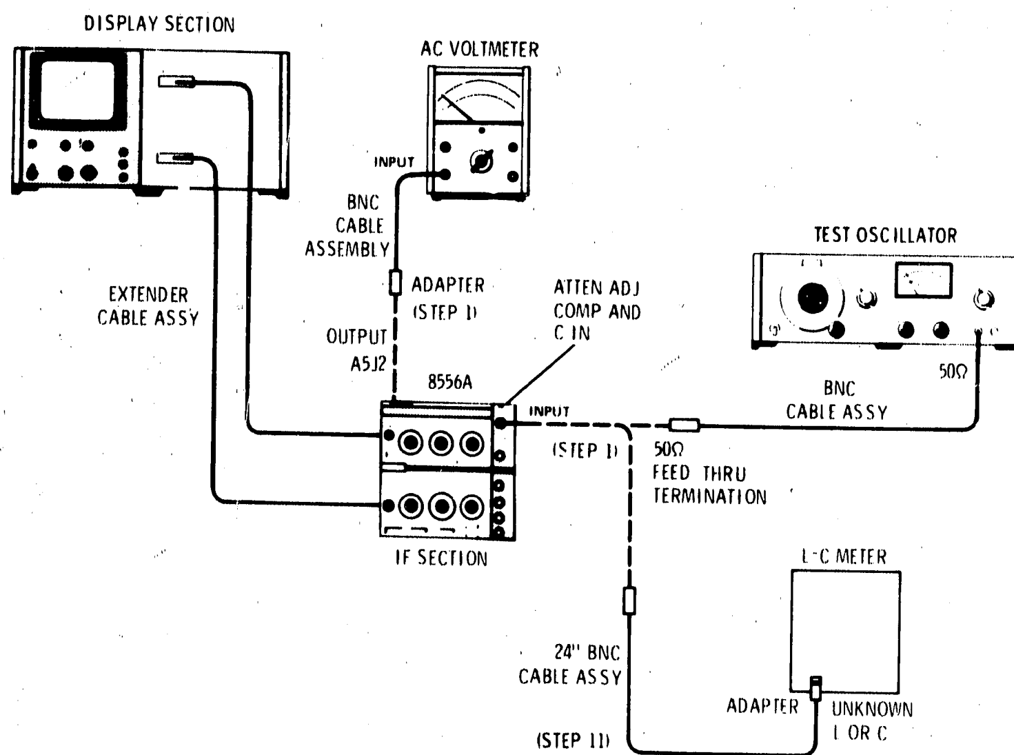
Figure 5-2. Pre-Attenuator Adjustment Test Setup
