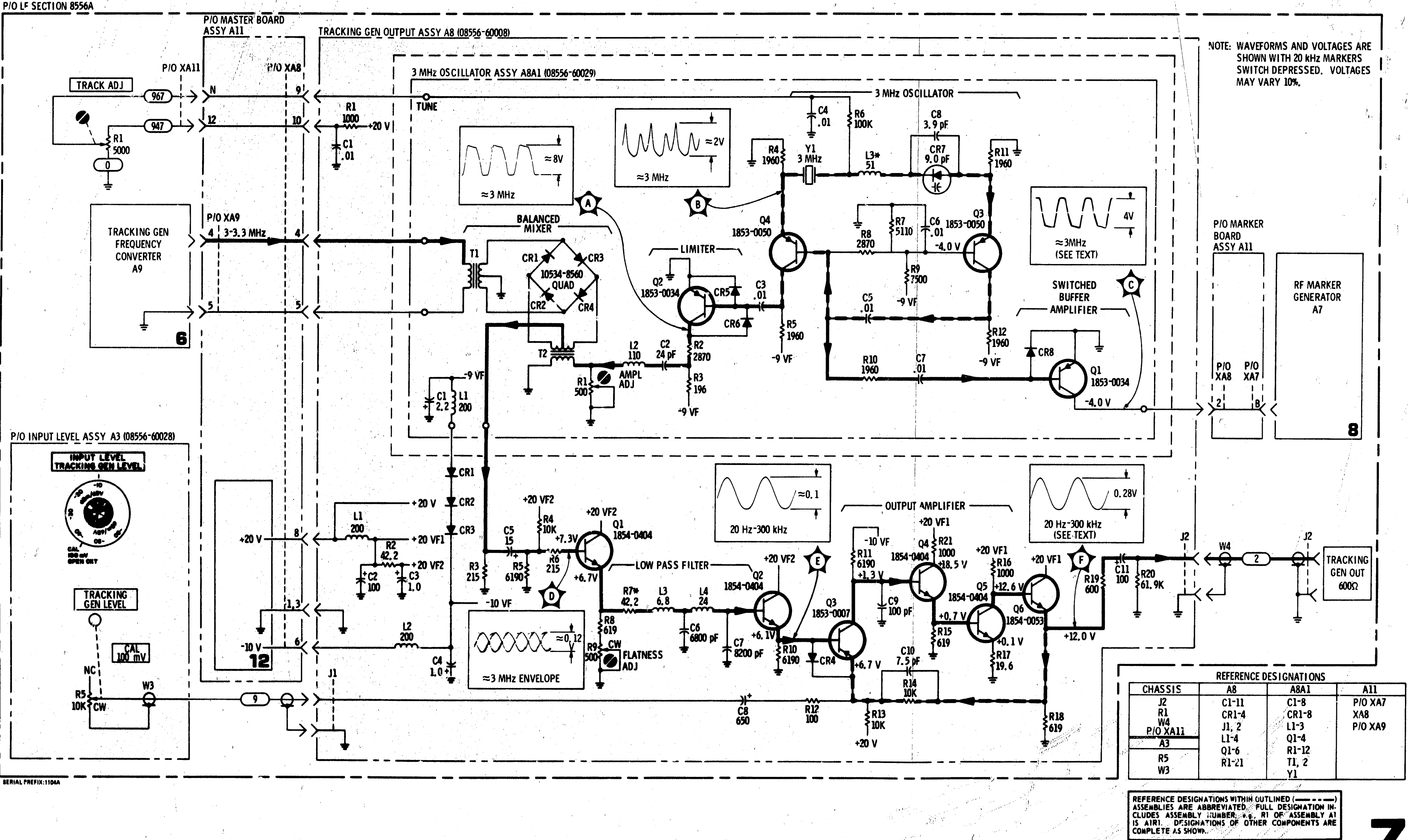
Figure 8-32. Tracking Generator Output: A3 and A8
