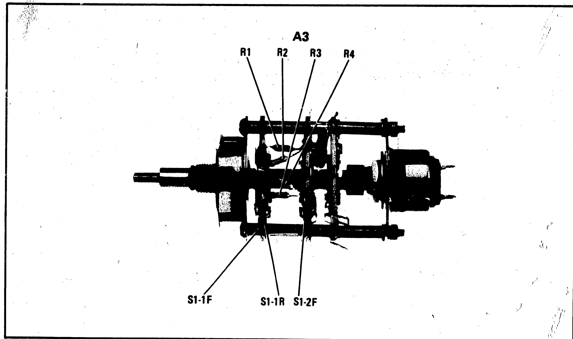
Figure 8-24. Input Level Switch Assembly A3 Component Locations
