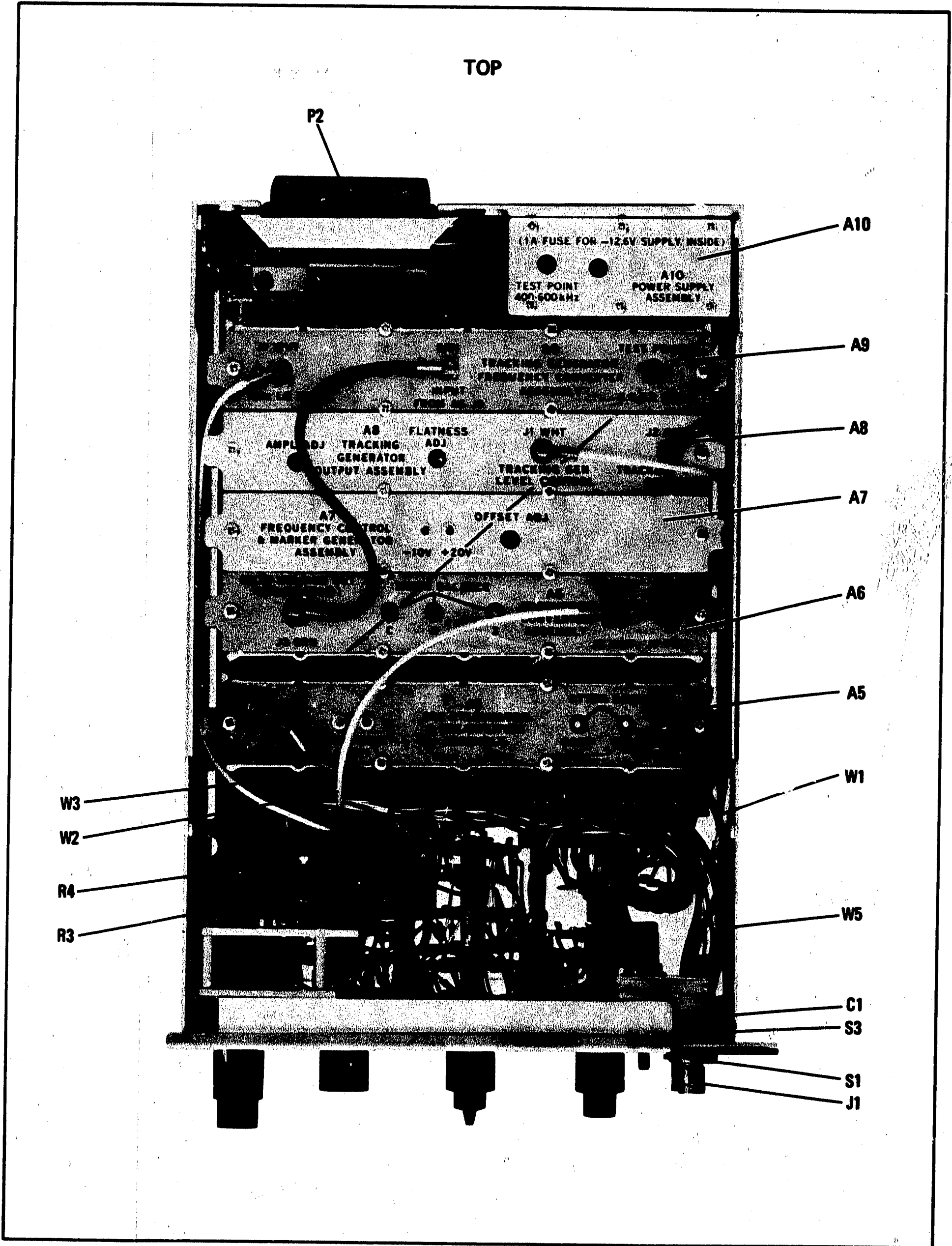
Figure 8-14. Top and Bottom Internal Views
