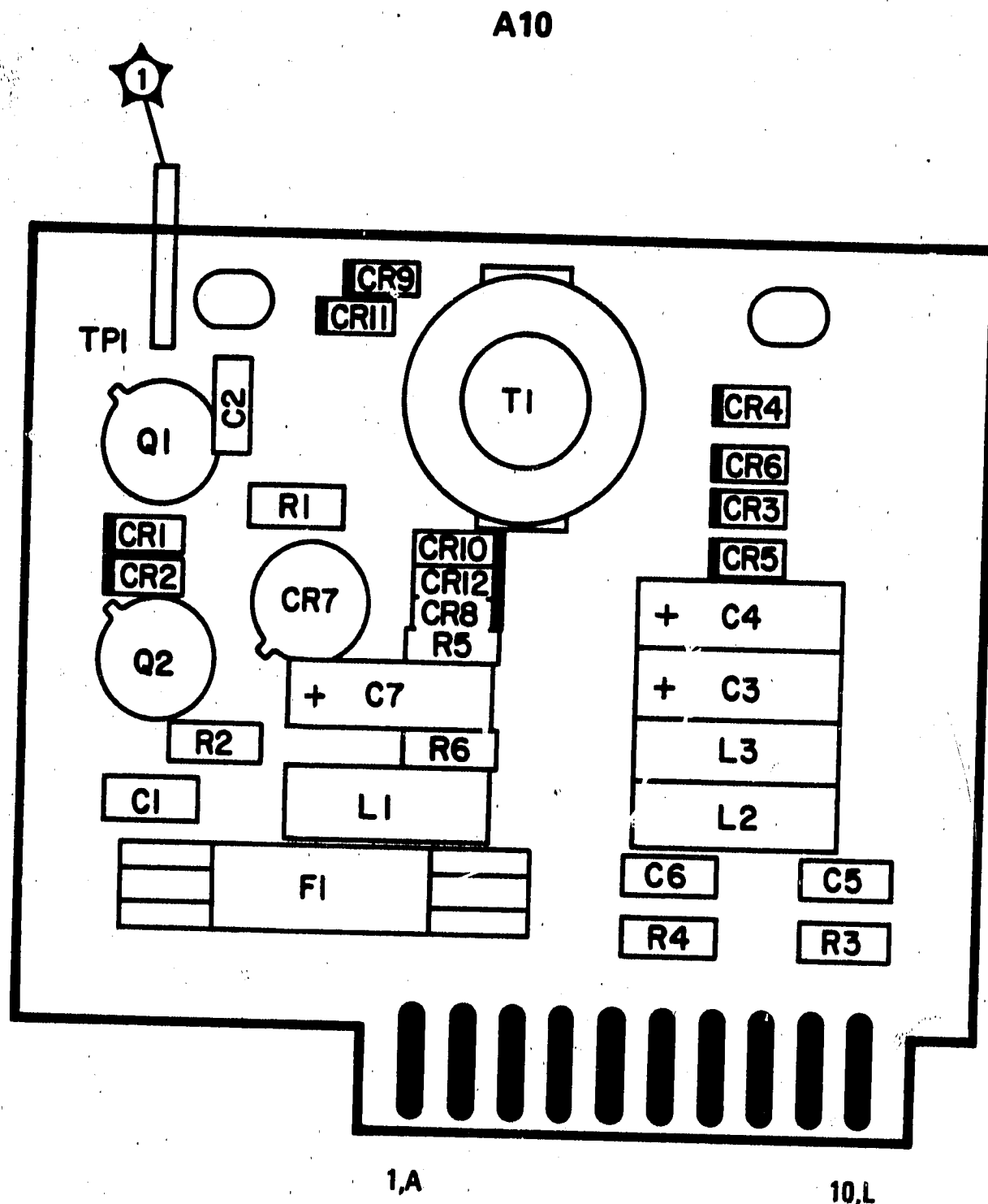
Figure 8-46. Power Supply Assembly A10 Component Locations (CHANGE 10)
