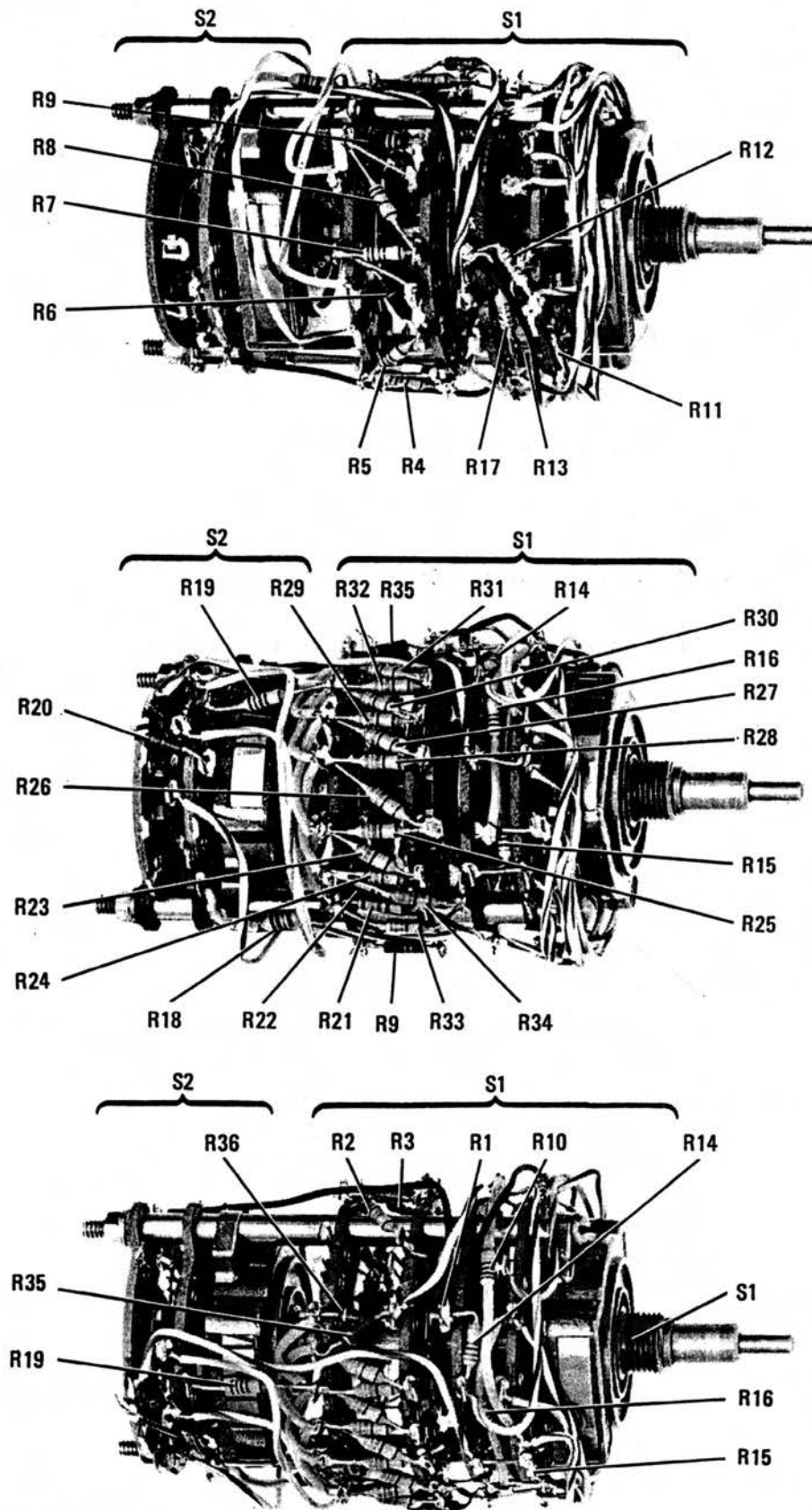
Figure 7-13. Scan Width Switch Assembly, A1A2, Figure 8-60 (Change M)
