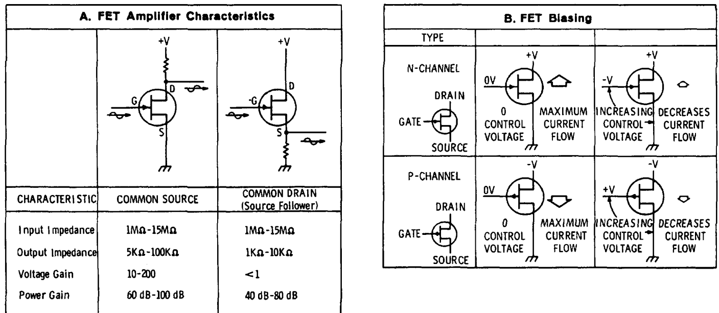
Figure 8-2. Field Effect Transistor Operation
