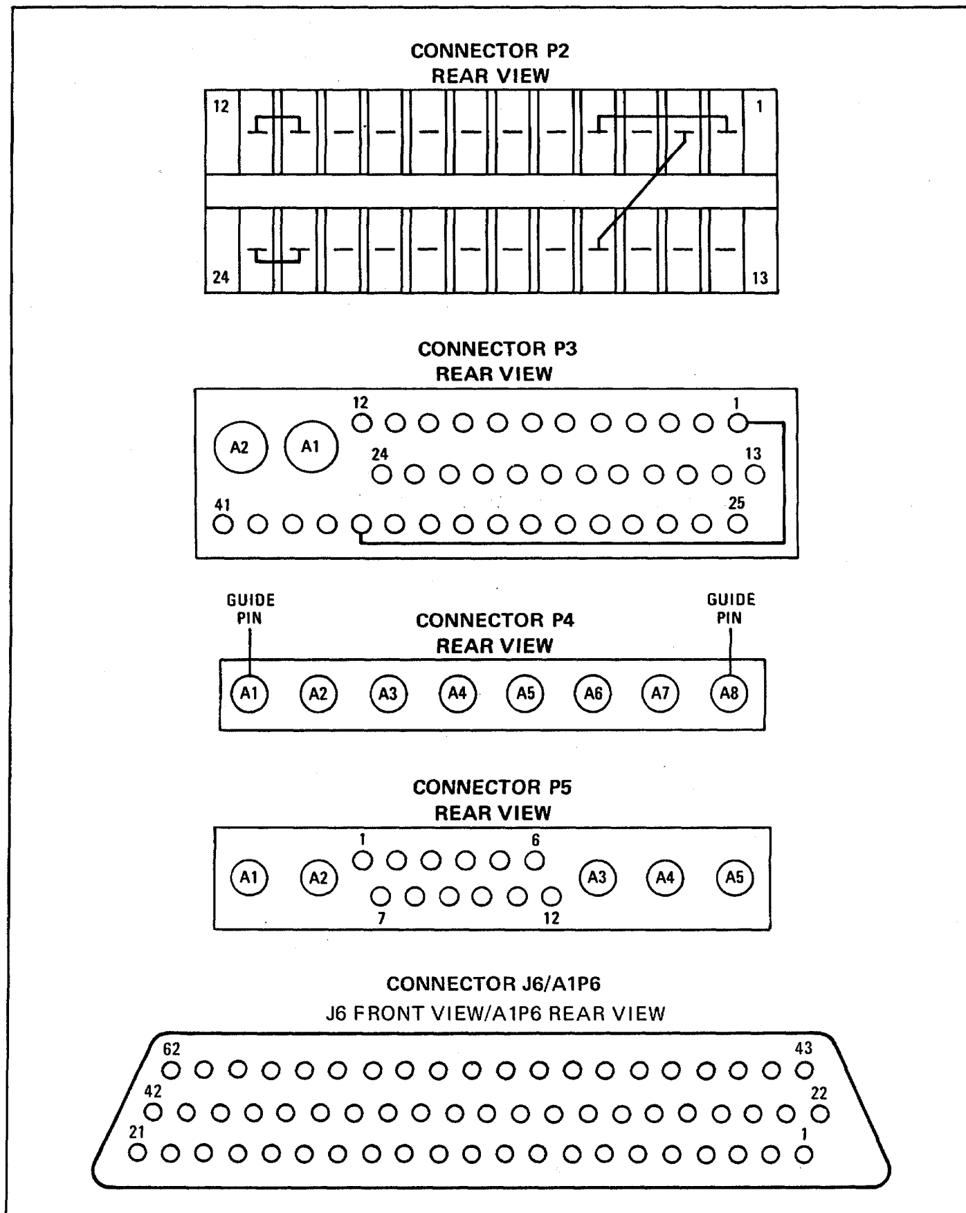
Figure 8-73. Connector Pin Location Diagram
