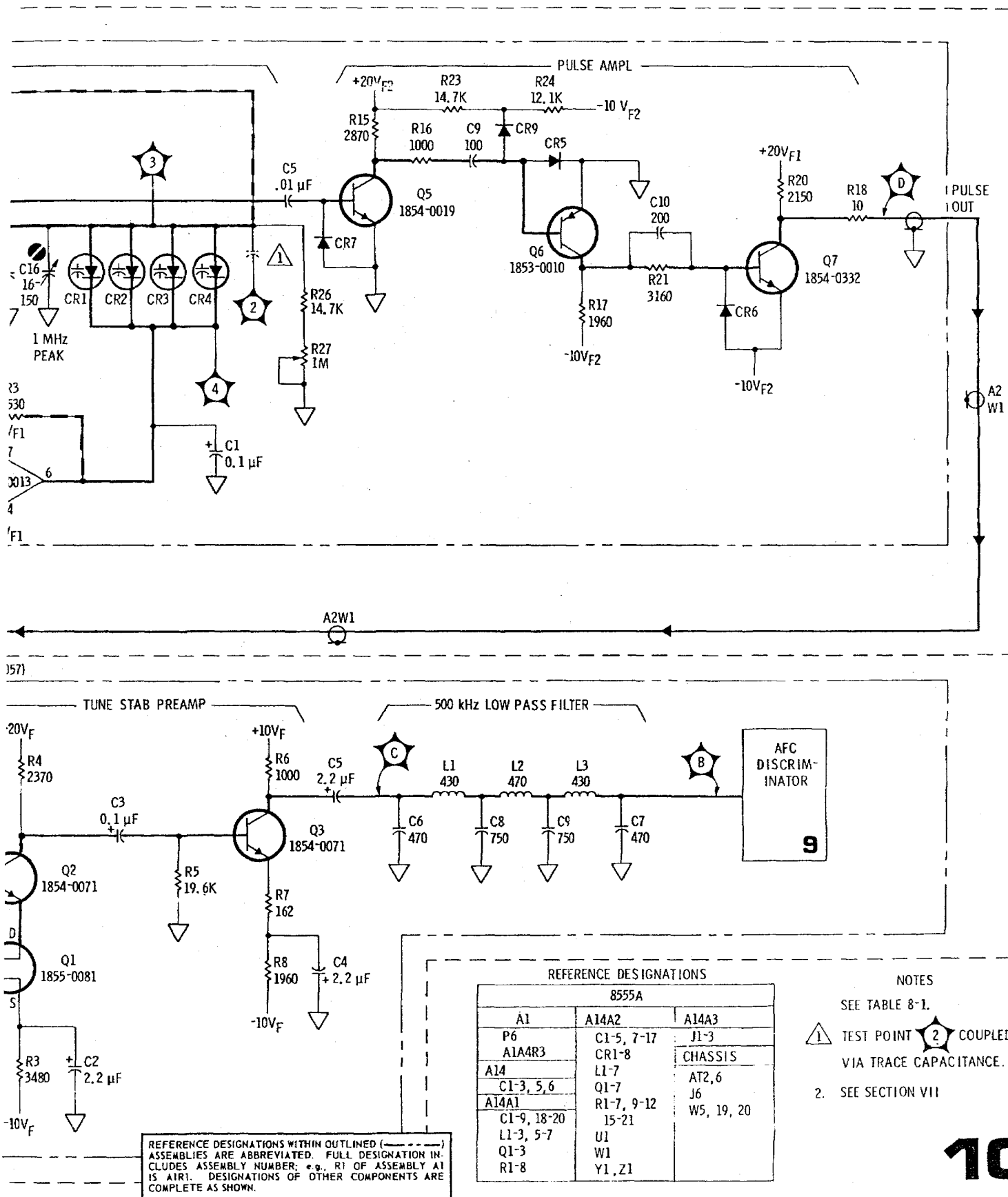
Figure 8-55. Tuning Stabilizer VCXO/Pulse Ampl Assy A14A2, Discriminator A14A1, and Sampler Assy A14A5
