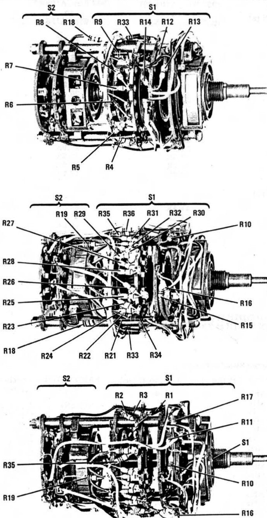
Figure 8-63. Scan Width Switch Assembly A1A2
