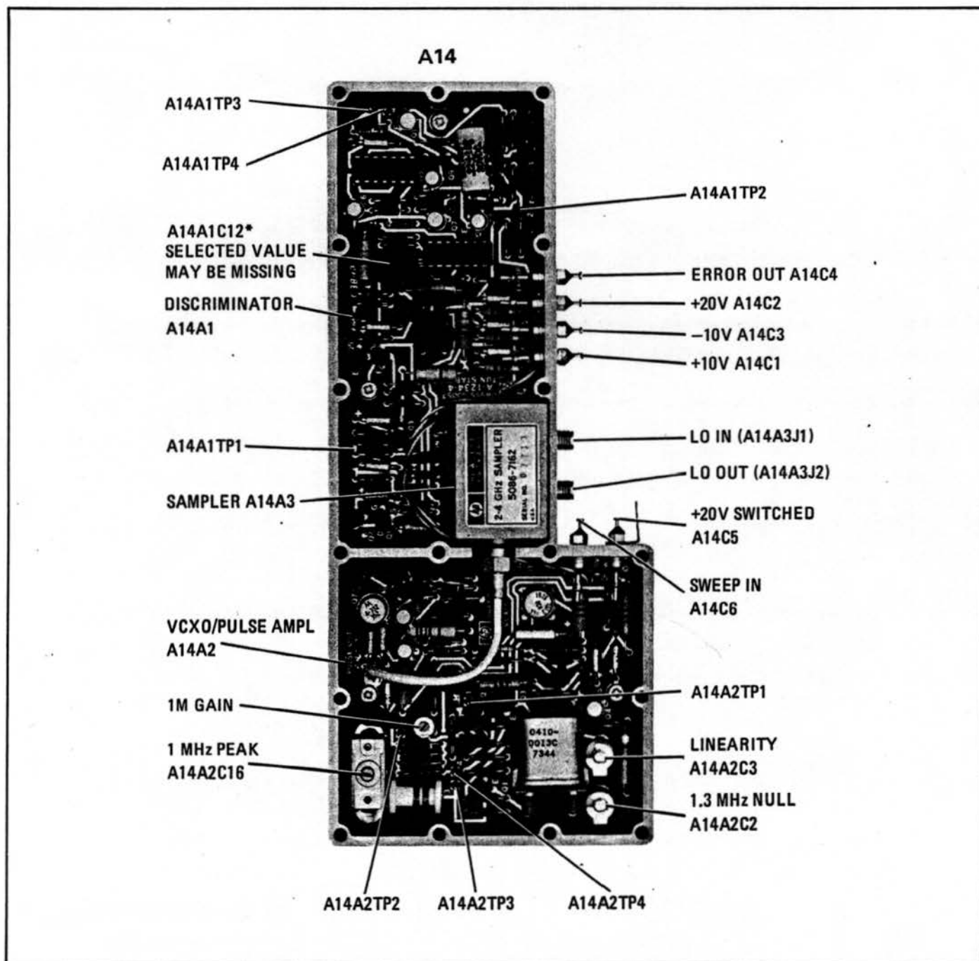
Figure 8-54. Tuning Stabilizer Assembly A14
