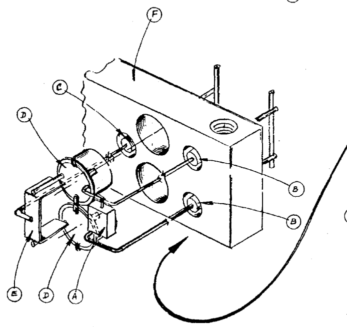
1T (22) OSC. ASS'Y 1.5 GHz
