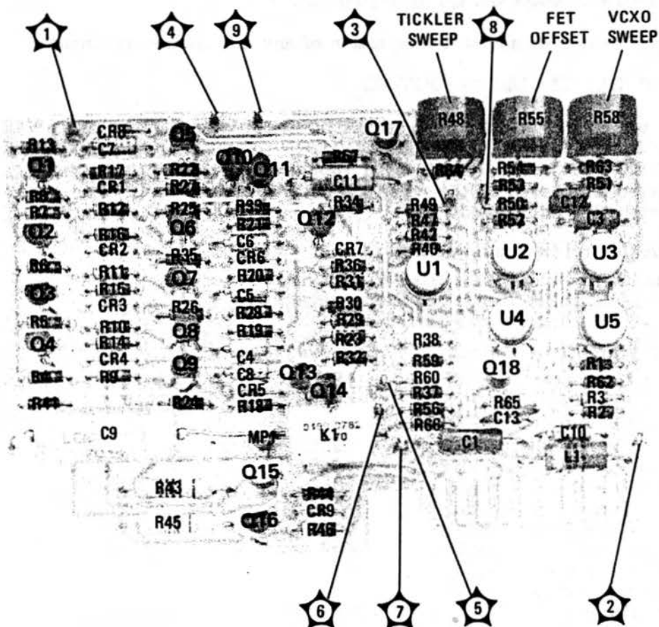
Figure 8-43. Tuning Stabilizer Control Assembly A5
