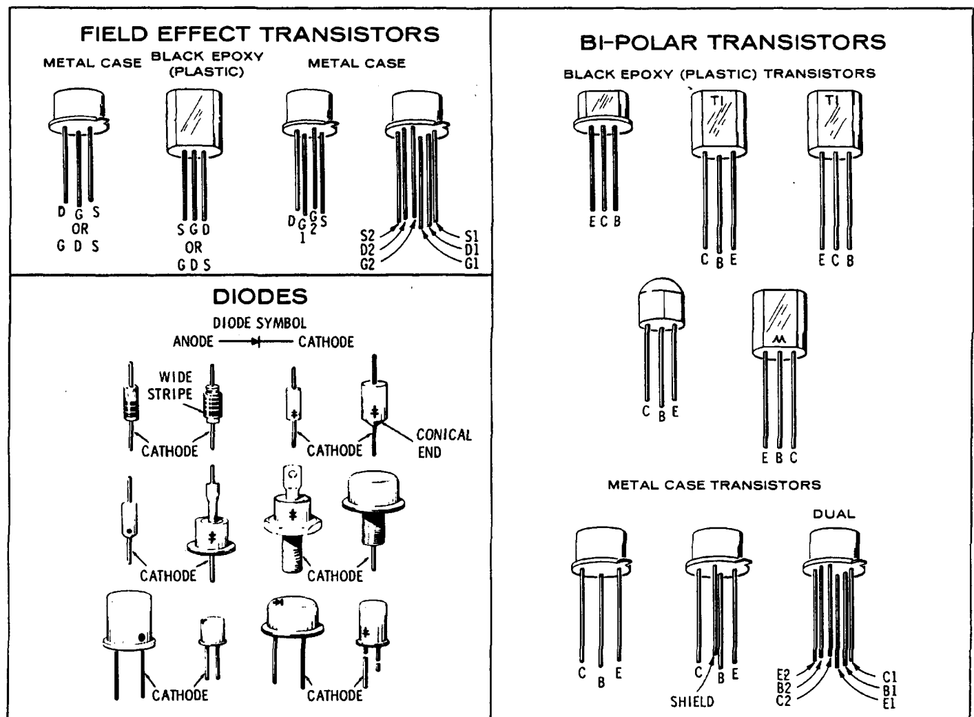
Figure 8-3. Examples of Diode and Transistor Marking Methods
