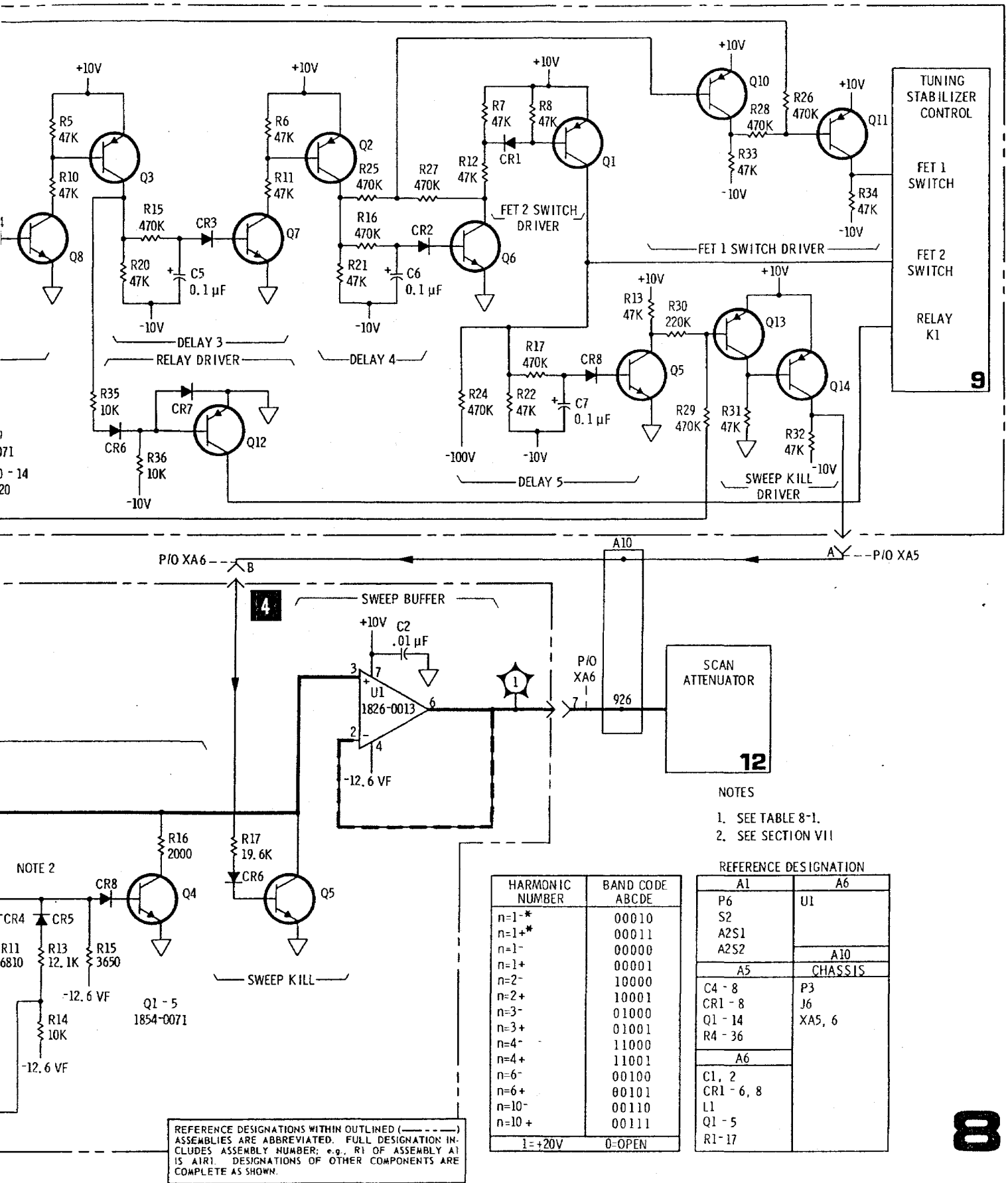
Figure 8-45. Control Generator and 1/n Attenuator
