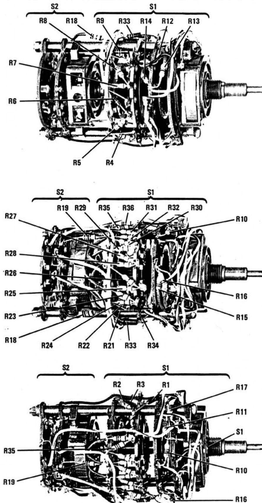
Figure 8-37. Scan Width Switch Assembly A1A2
