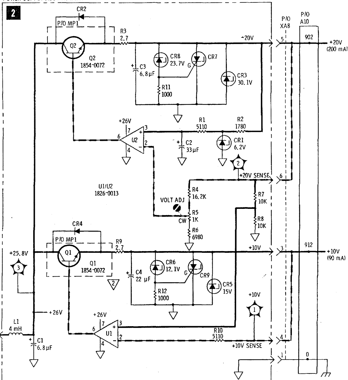
POWER SUPPLY ASSY A8 (08555-60055)
