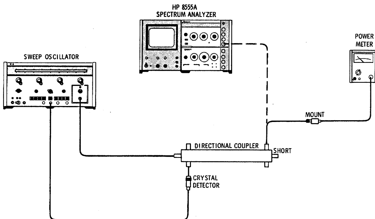
Figure 4-6. Frequency Response Test Setup, 0.1 to 2.05 GHz
