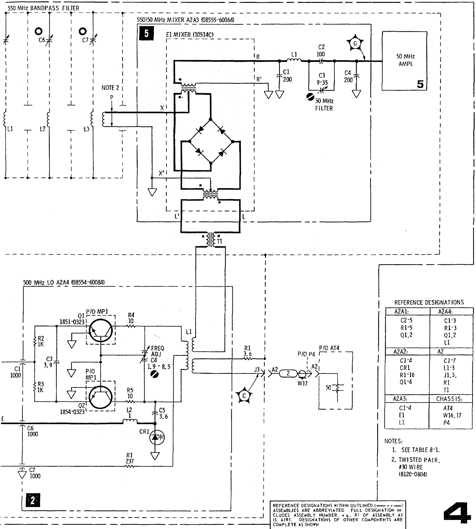
Figure 8-28. Third Converter
