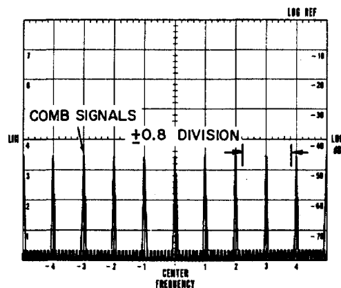
Figure 4-4. Scan Width Accuracy Measurement
