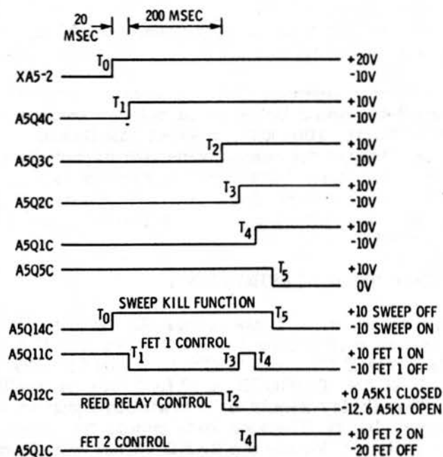
Figure 8-42. Control Generator Timing Diagram
