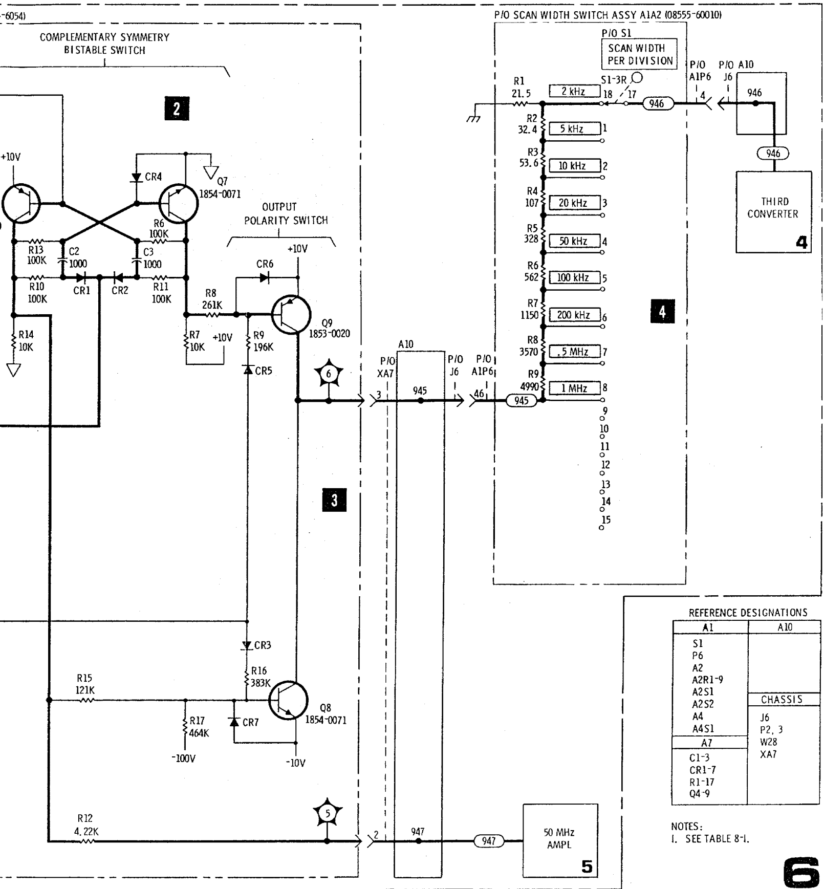
Figure 8-38. Signal Identifier
