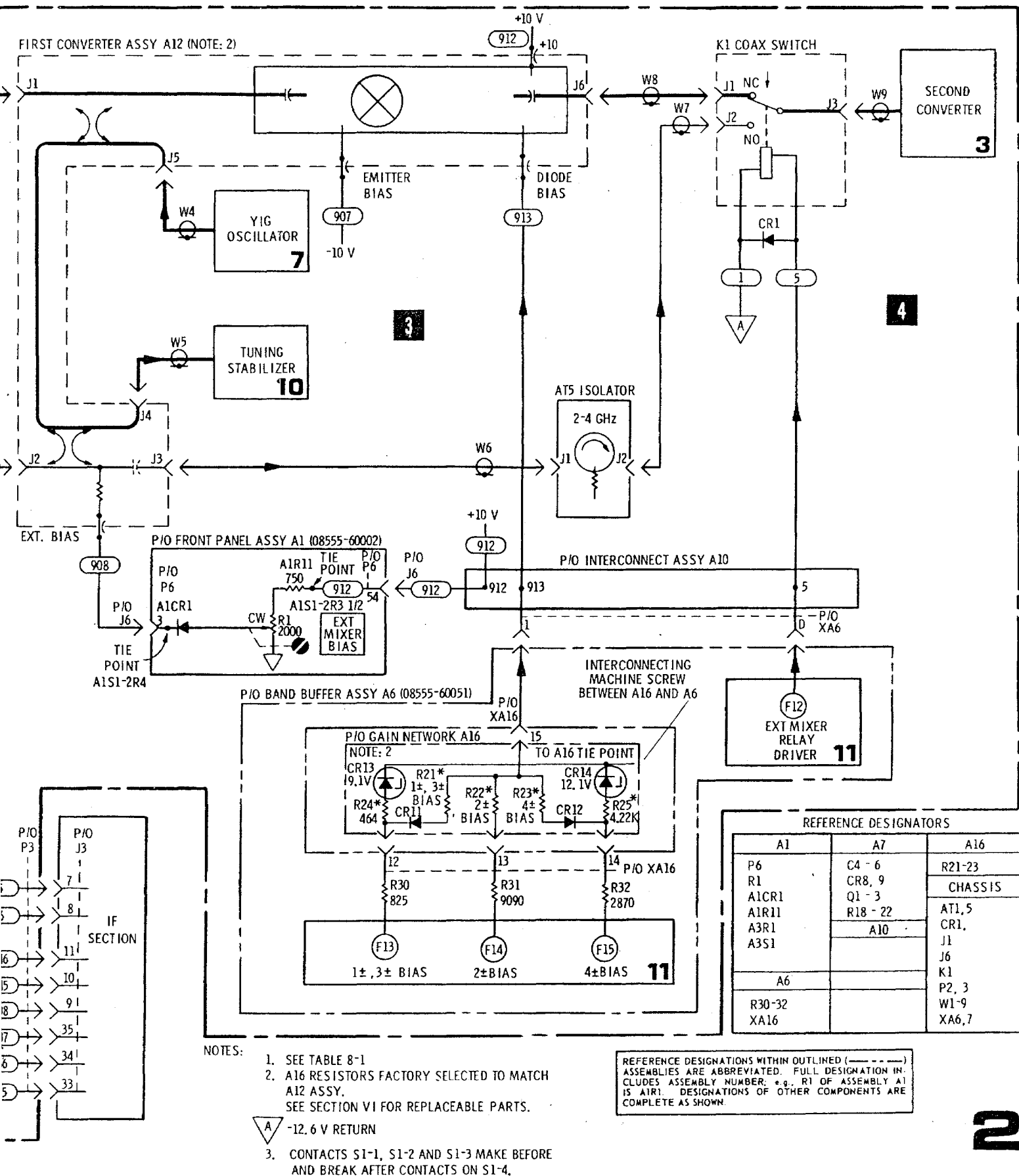
Figure 8-17. Input Attenuator and 1st Converter Schematic Diagram
