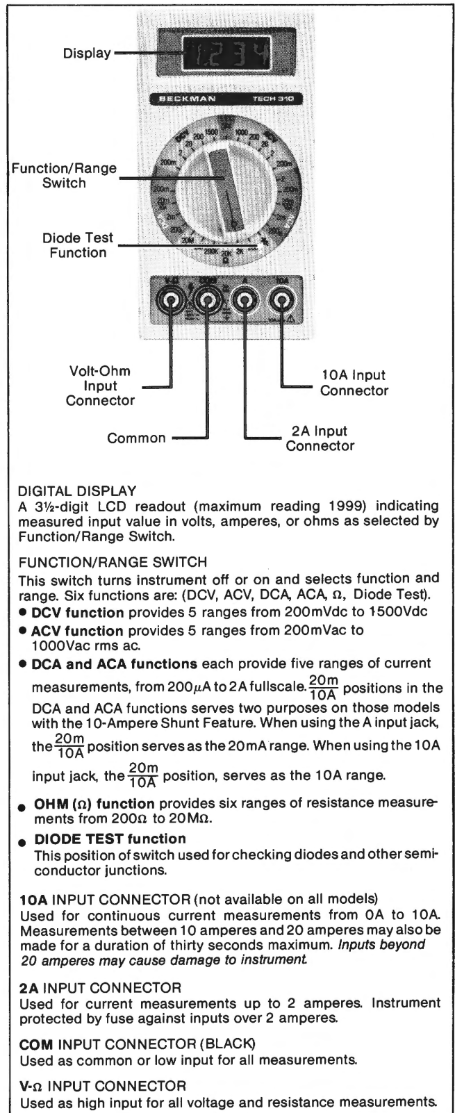
Figure 4-1. Operating Controls and Input Connectors
