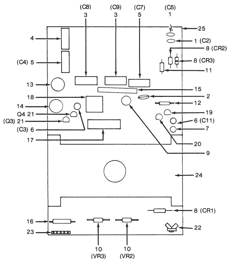
Figure 5-8. Large Circuit Board Assembly (3010, 3020, TECH 300, TECH 310) for Part Location
