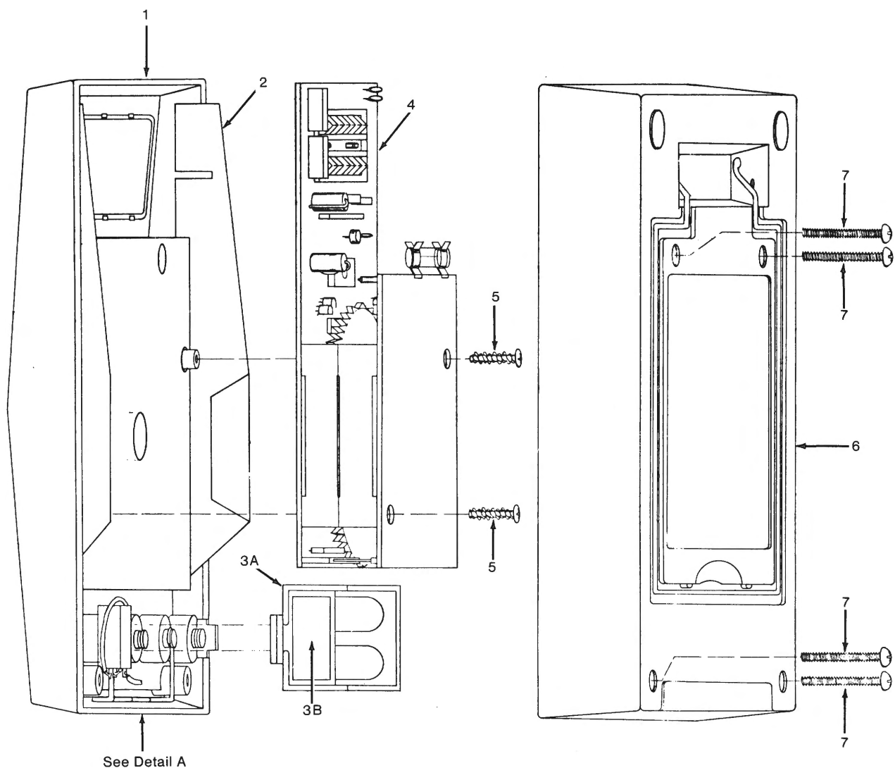
Figure 5-1. Multimeter Assembly
