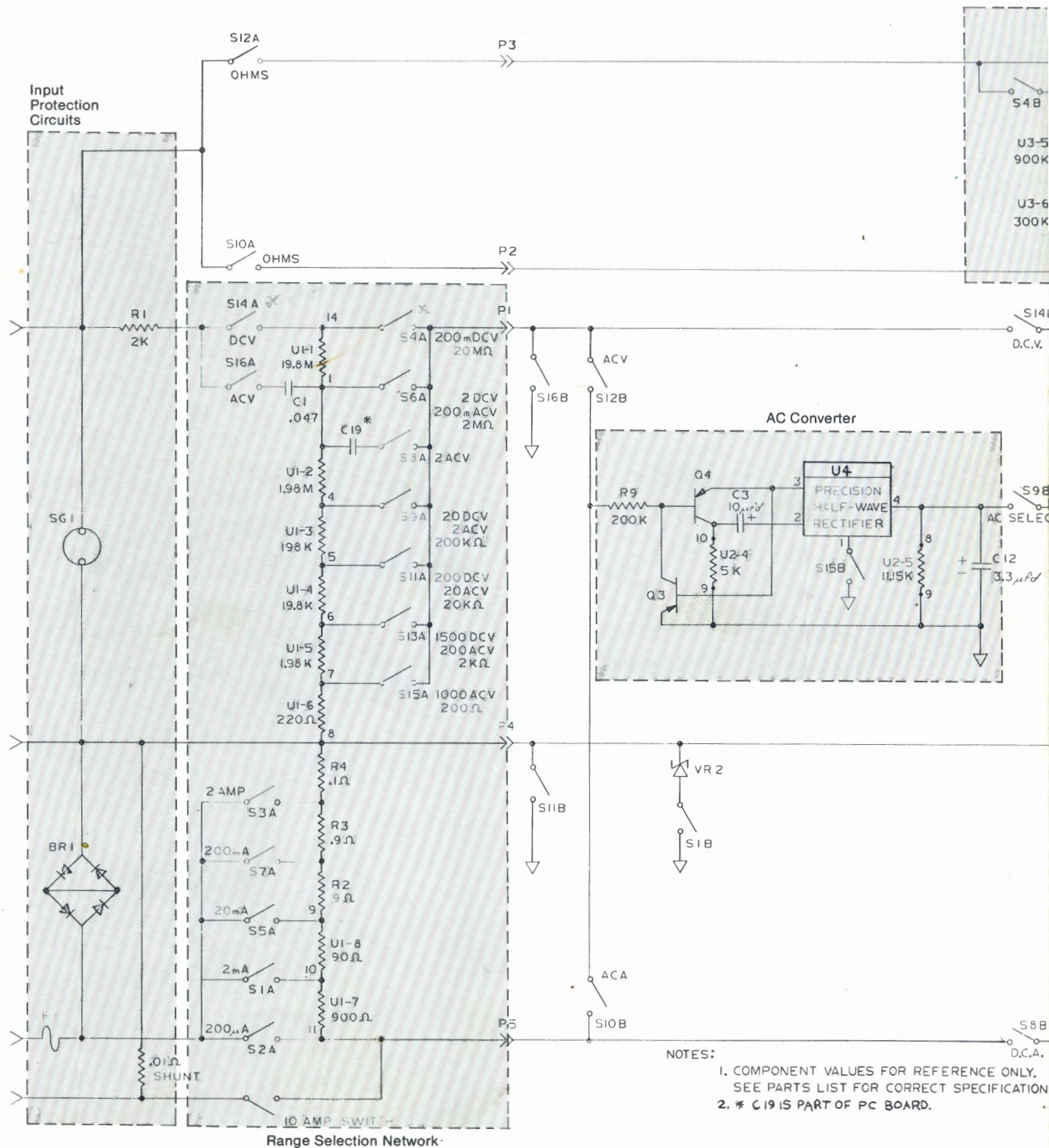
Figure 4-3A. Multimeter Schematic Diagram (TECH 300, TECH 310, 3010, 3020)
