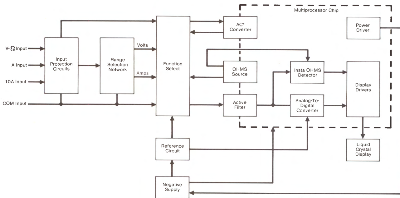
Figure 2-1. Multimeter Simplified Block Diagram
