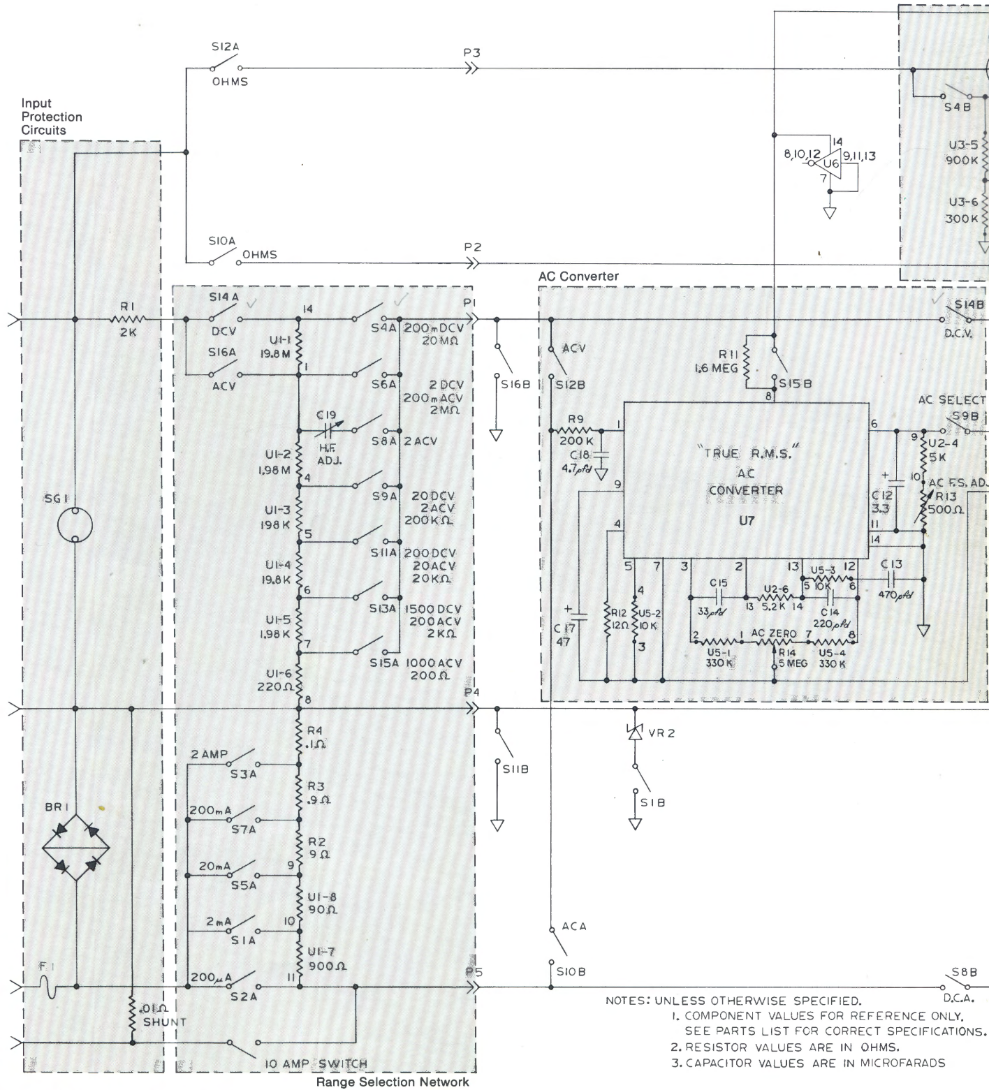
Figure 4-3B. Multimeter Schematic Diagram (RMS 3030, TECH 330)
