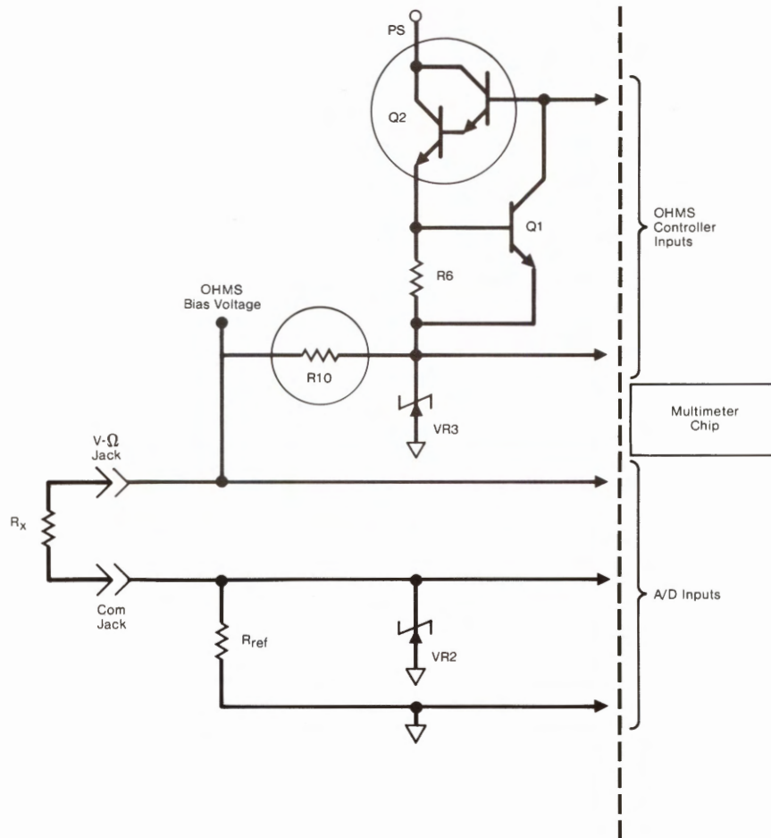
Figure 2-3. Circuit for Resistance Measurements
