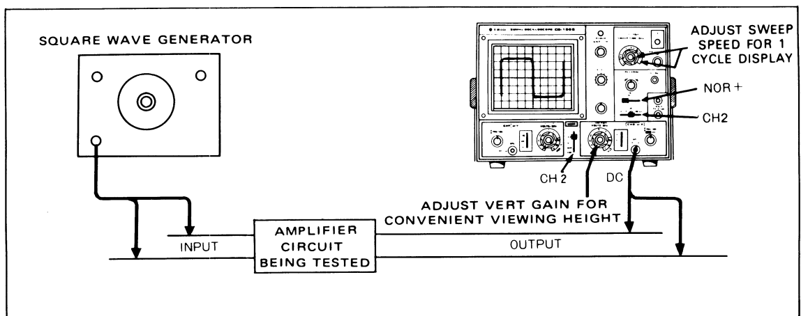
Fig. 28 Equipment set-up for square wave testing of amplifiers
