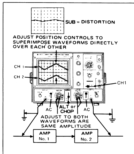
Fig. 10 Distortion measurement
