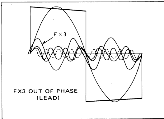
Fig. 33 Square wave tilt resulting from 3rd harmonic phase shift
