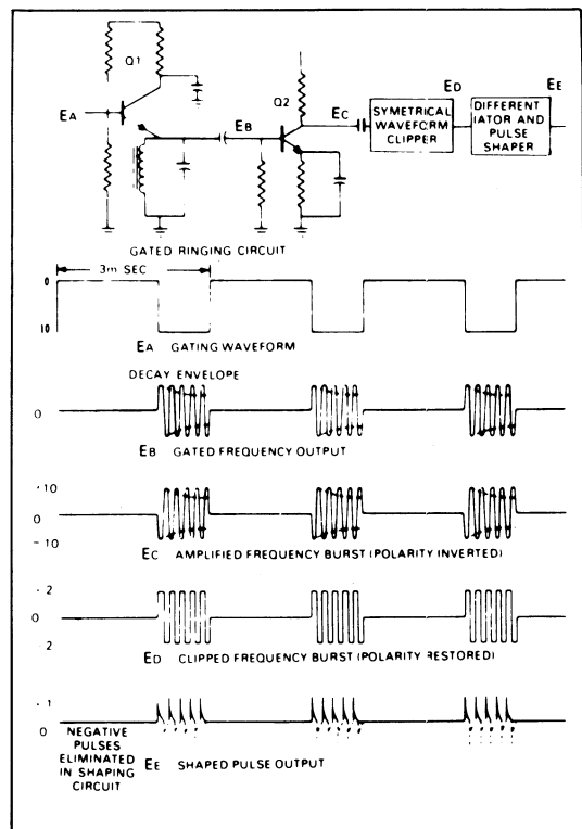
Fig. 11 Gated ringing circuit and waveforms
