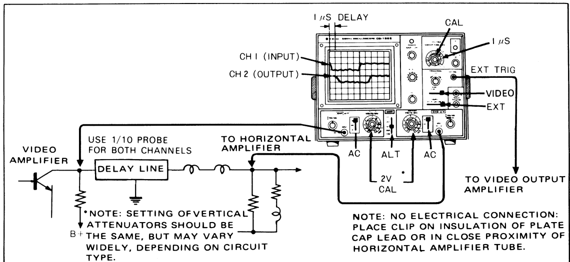
Fig. 13 Checking "Y" delay line in color television receivers
