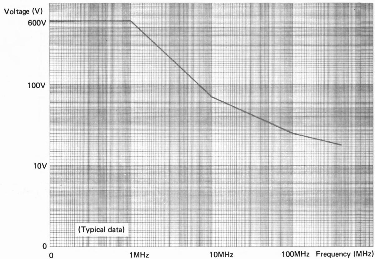
Figure 1. Input voltage
