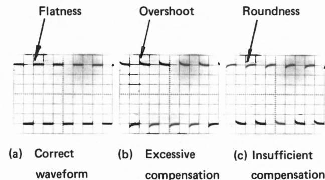
Figure 3. Waveform of low-frequency phase
