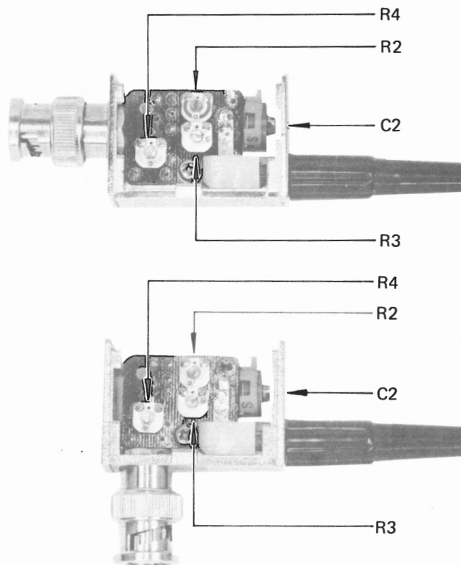
Figure 8. Controls in matching-box (2)
