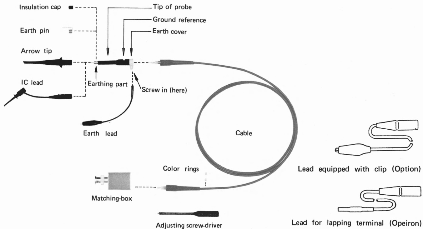
Figure 2. (1) Straight form probe unit and its standard/option accessories
