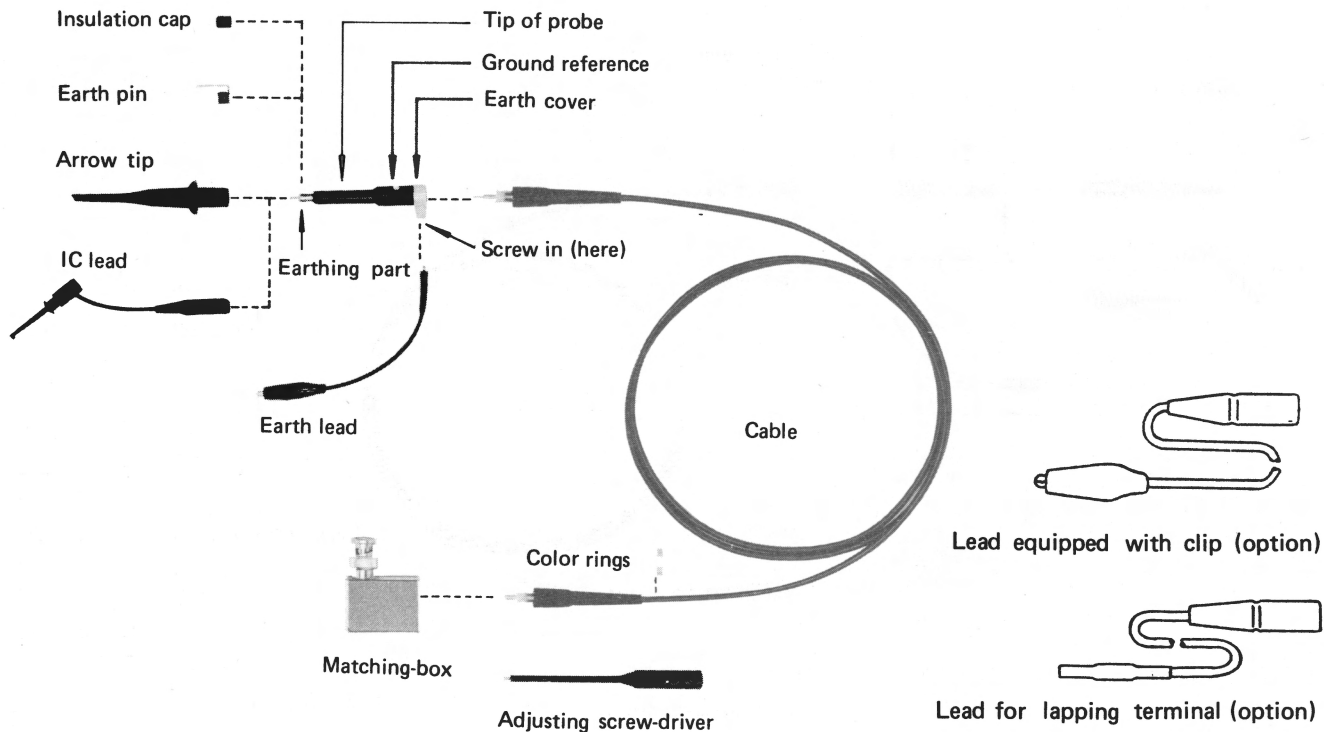
Figure 2. (2) L-shaped probe unit and its standard/option accesories
