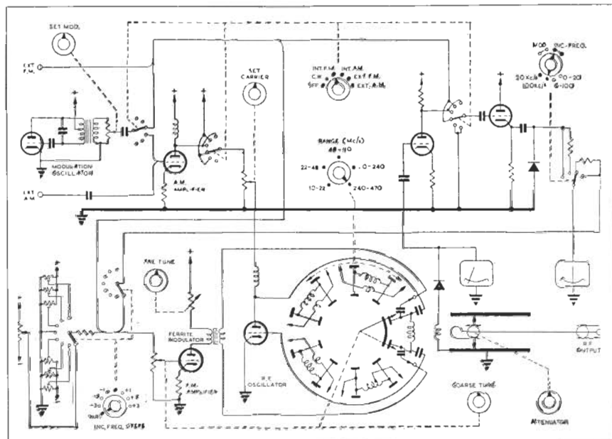
Functional Diagram of TF 1066B
