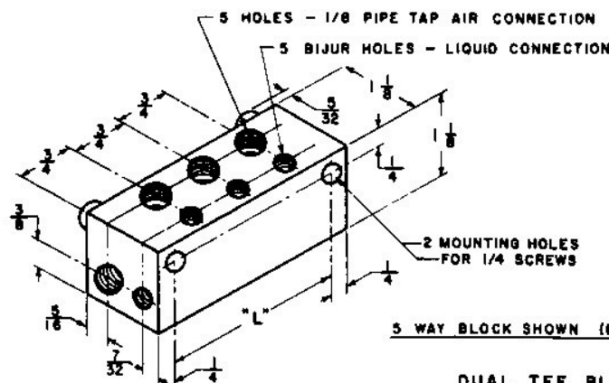
DUAL TEE BLOCKS
