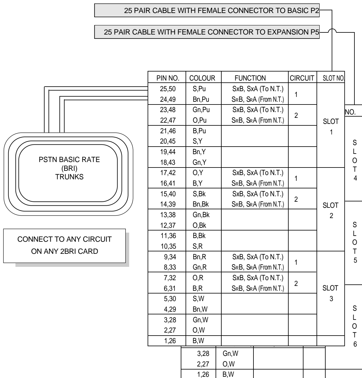
&lt;FIGURE 5-7&gt; MDF CONNECTIONS FOR ISDN C.O LINE TO CARD (2BRI)
