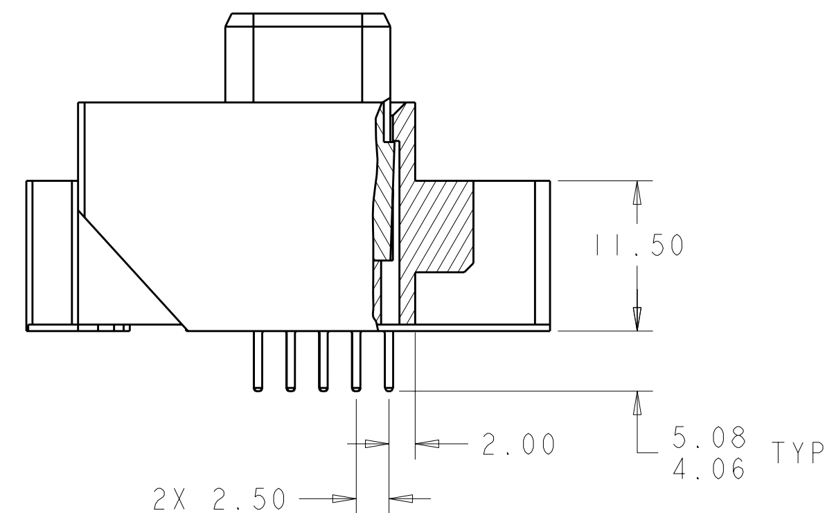
SECTION Z-Z
