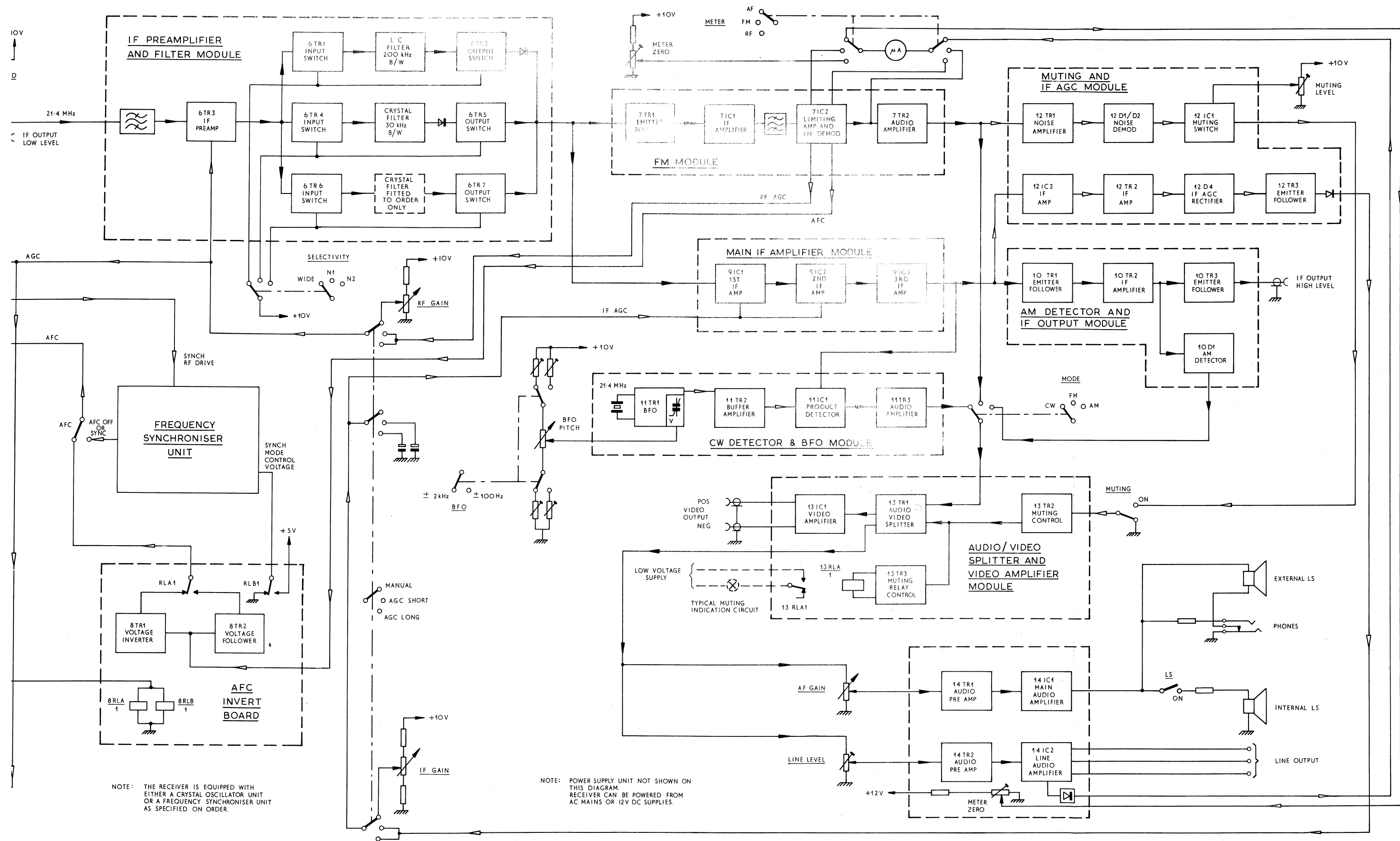
BLOCK DIAGRAM
