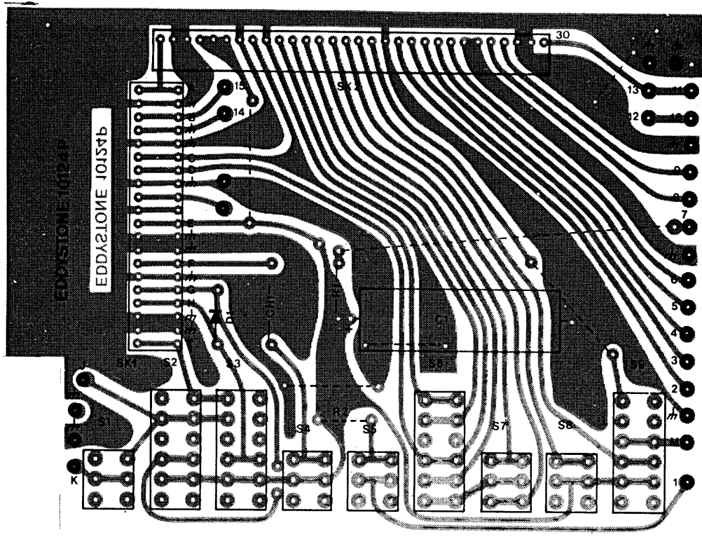
(4) CONTROL BOARD
