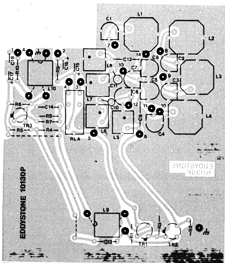
(5) AERIAL AMPLIFIER
