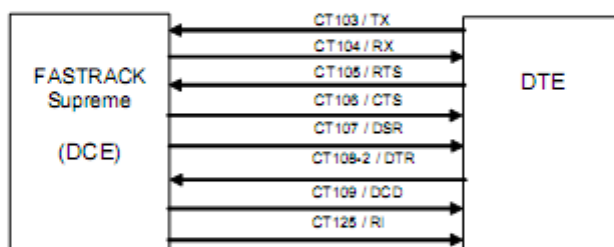
Figure 16: RS232 Serial Link signals
