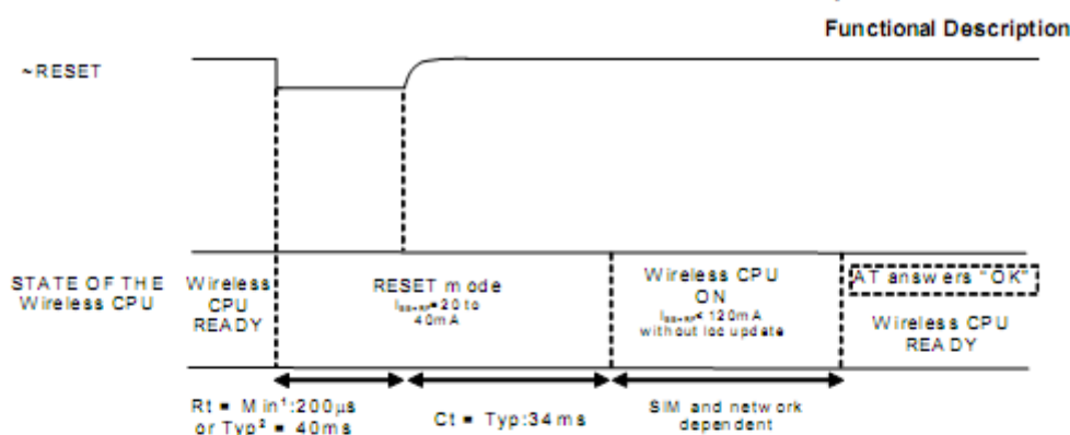
Figure 17: Reset sequence diagram
