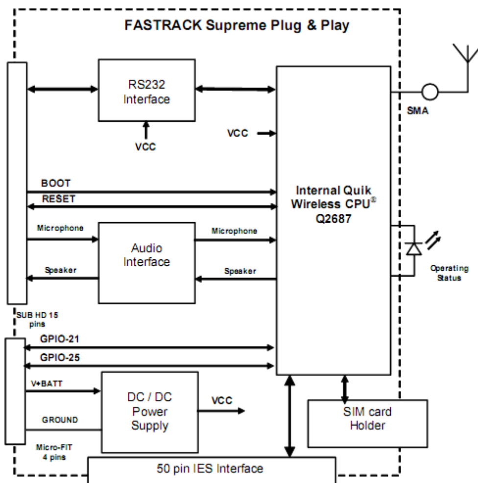
Figure 15: Functional architecture
