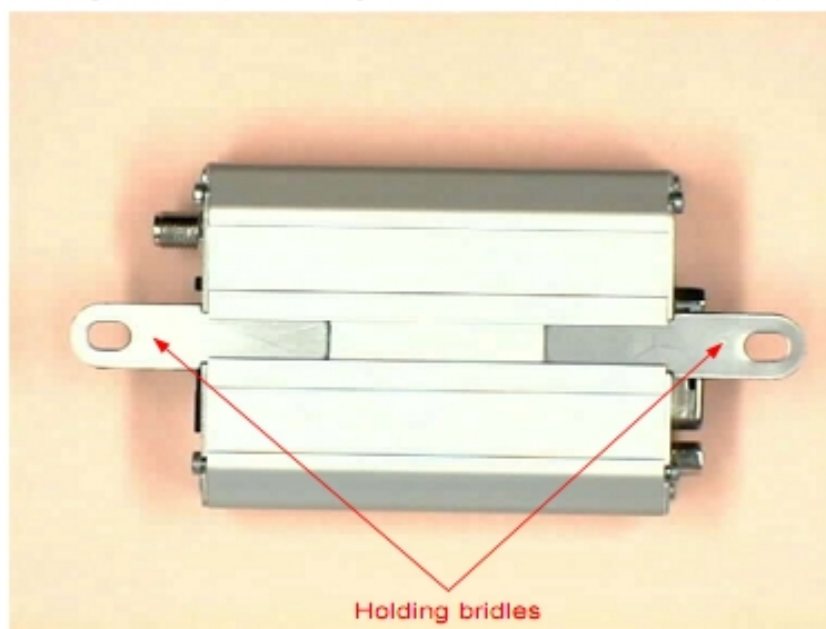
Figure 5: FASTRACK Supreme holding bridles
