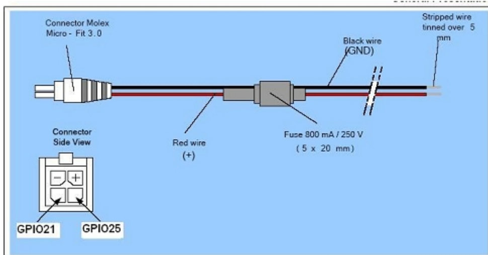
Figure 10: Power supply cable
