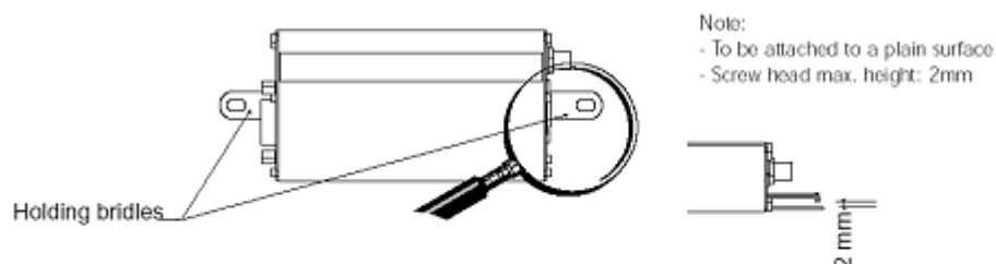
Figure 12: FASTRACK Supreme mounting
