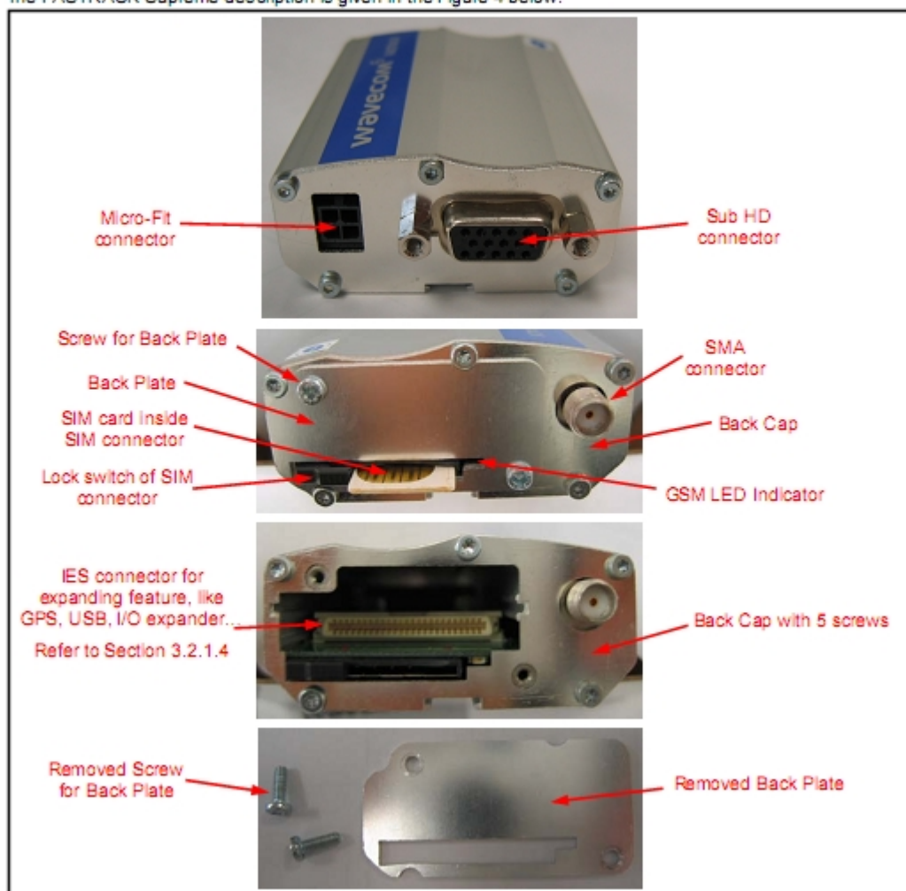
Figure 4: FASTRACK Supreme general description
