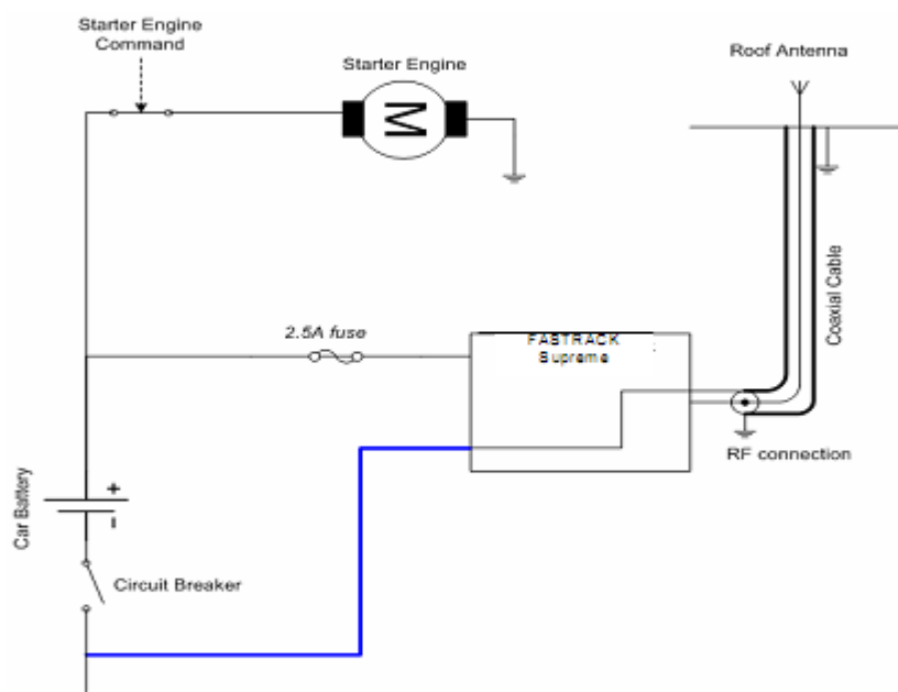
Figure 13: Recommended power supply connection on trucks
