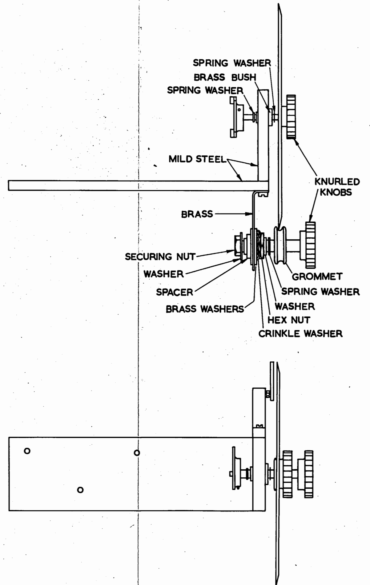
FIG.15.1 OSCILLATOR ADJUSTMENT TEST JIG.
