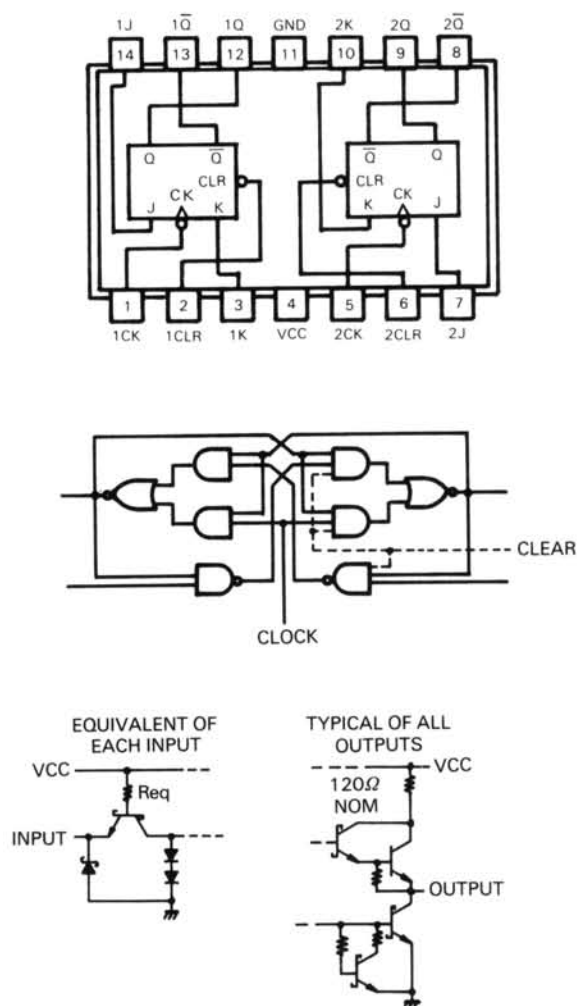
Fig. 6 SN74LS73N (PLL unit IC1)
