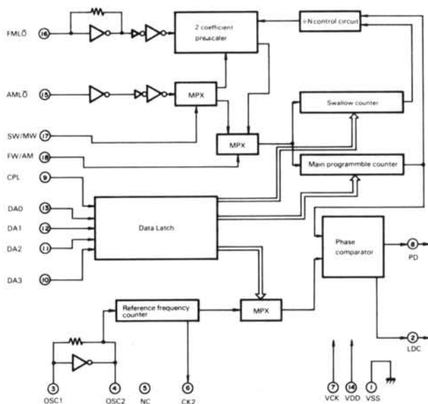
Fig. 7 MN6147C (PLL unit IC2, 5)
