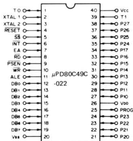
Fig. 12. \mu\text{PD80C49C-022} Terminal name
