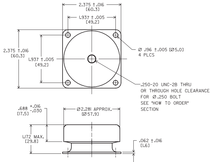
SERIES 1000 Dimensional Drawing
