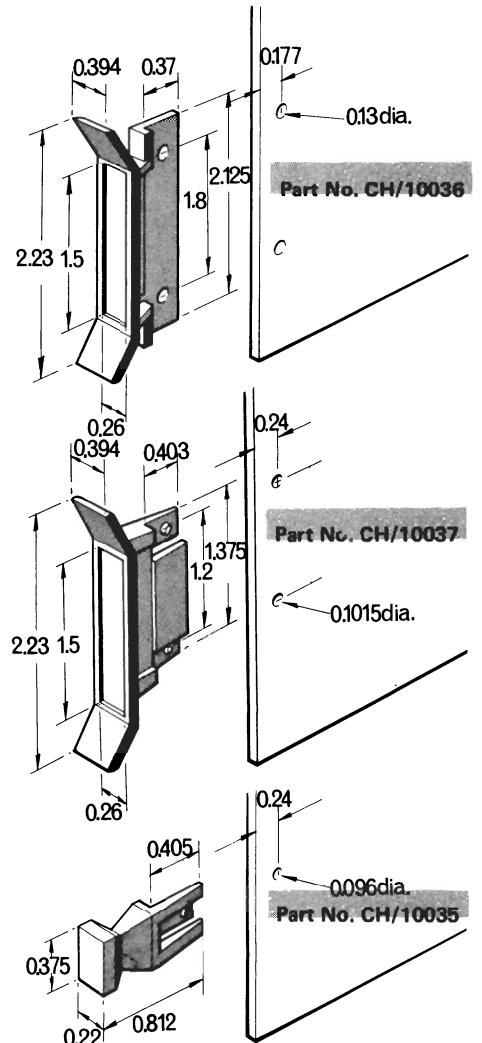
Insertion method types B.C & F
