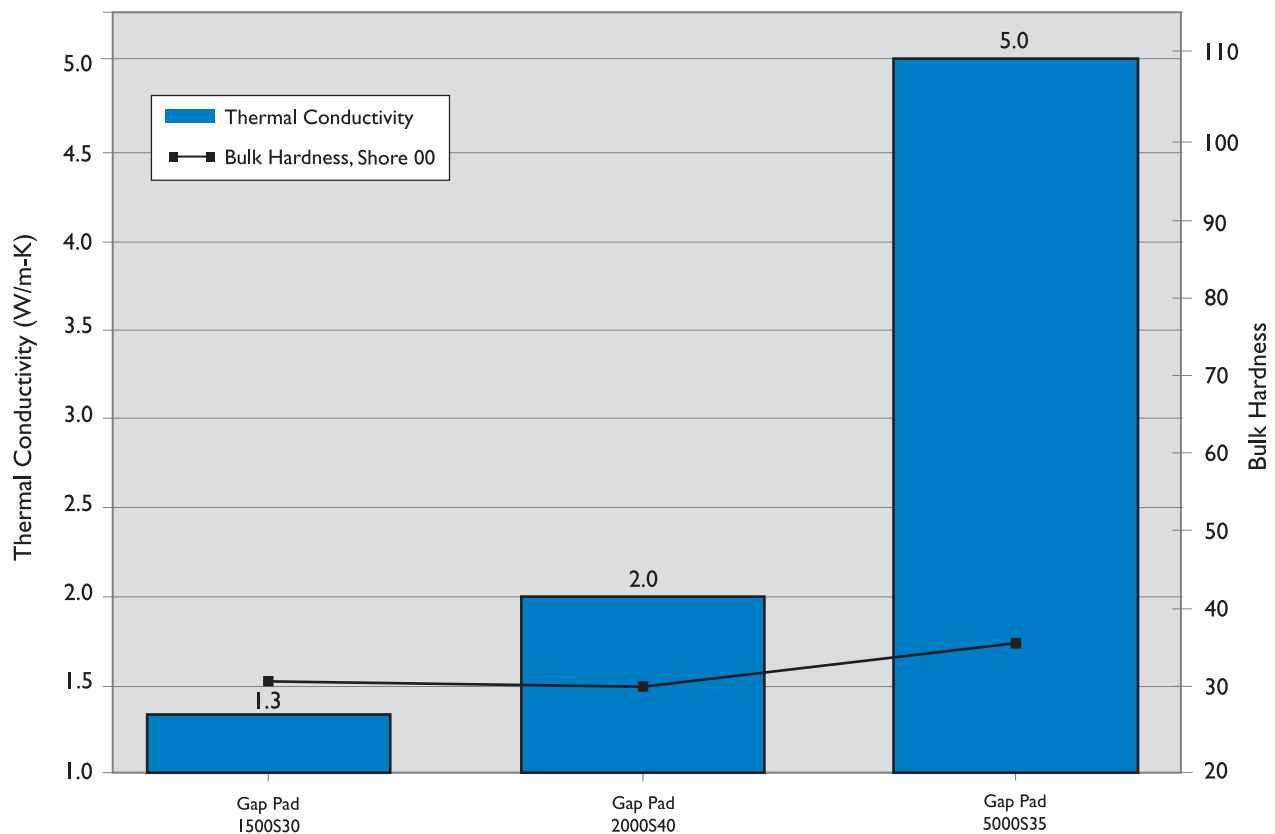
Gap Pad "S-Class" Thermal Conductivity vs. Hardness
