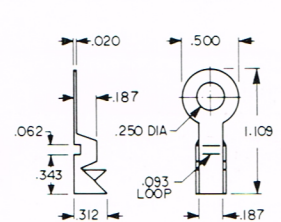
CAT. NO. 7339 MATERIAL: .020 Copper, Tin Plate
