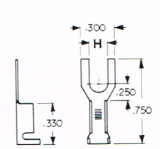
CAT. NO. 7339 MATERIAL: .020 Copper, Tin Plate
