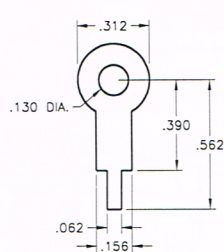
CAT. NO. 680 MATERIAL: .015 Brass, Tin Plate
