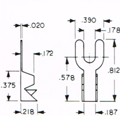
CAT. NO. 7337 MATERIAL: .020 Copper, Tin Plate
