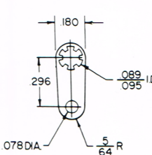
CAT. NO. 907 MATERIAL .013 Brass, Tin Plate
