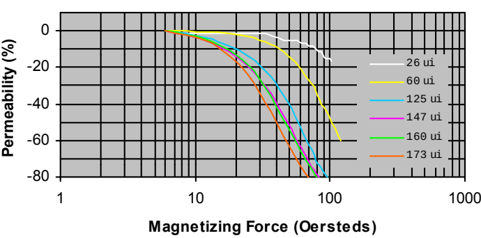
Inductance vs DC Bias at 200 gauss, 1kHz
