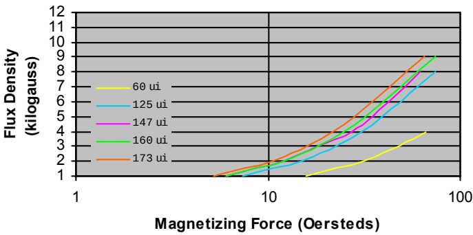
Magnetization Curves
