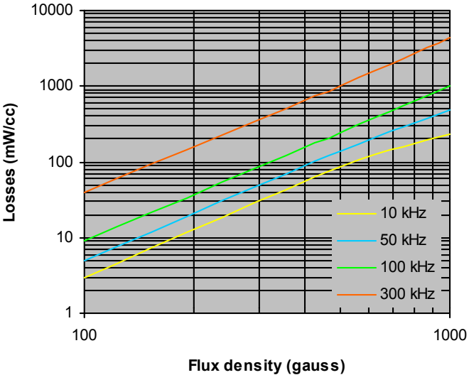
Power Loss Density vs Flux Density -93 Material grade, ui = 60
