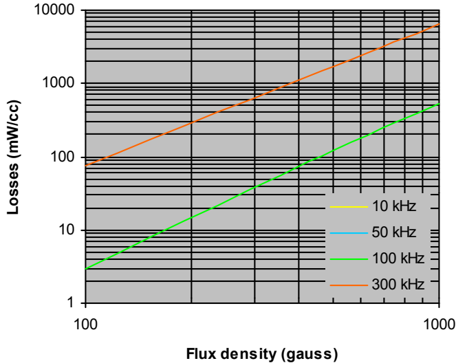
Power Loss Density vs Flux Density -92 Material grade, ui = 26
