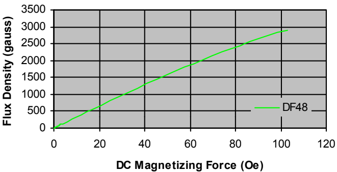
Normal Magnetizing Curve
