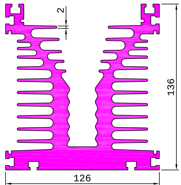
26357 16.282 kg/m
