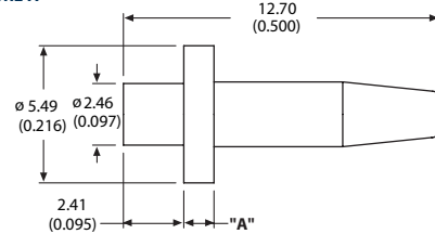
Pin P2-P3
