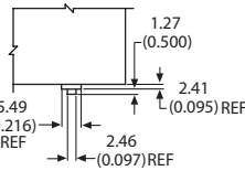
Pin P2-P3
