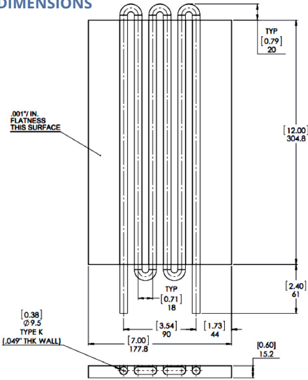
MECHANICAL DIMENSIONS
