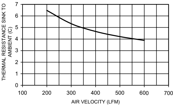
607 THERMAL PERFORMANCE
