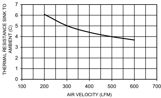
602 THERMAL PERFORMANCE
