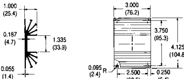
641 SERIES (EXTRUSION PROFILE 1371)
