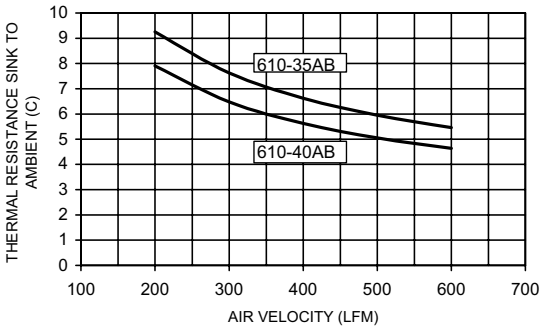
610 THERMAL PERFORMANCE
