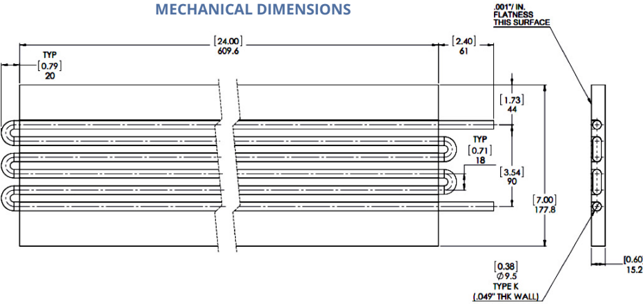
MECHANICAL DIMENSIONS
