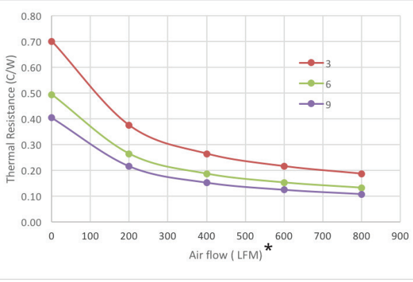
THERMAL RESISTANCE FOR 3", 6", 9" CUT LENGTHS
