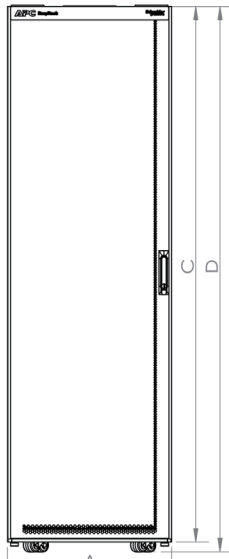
Front view
