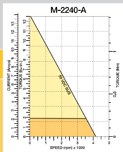
Page9 Baldor's DC Servo Motors Performance Curves
