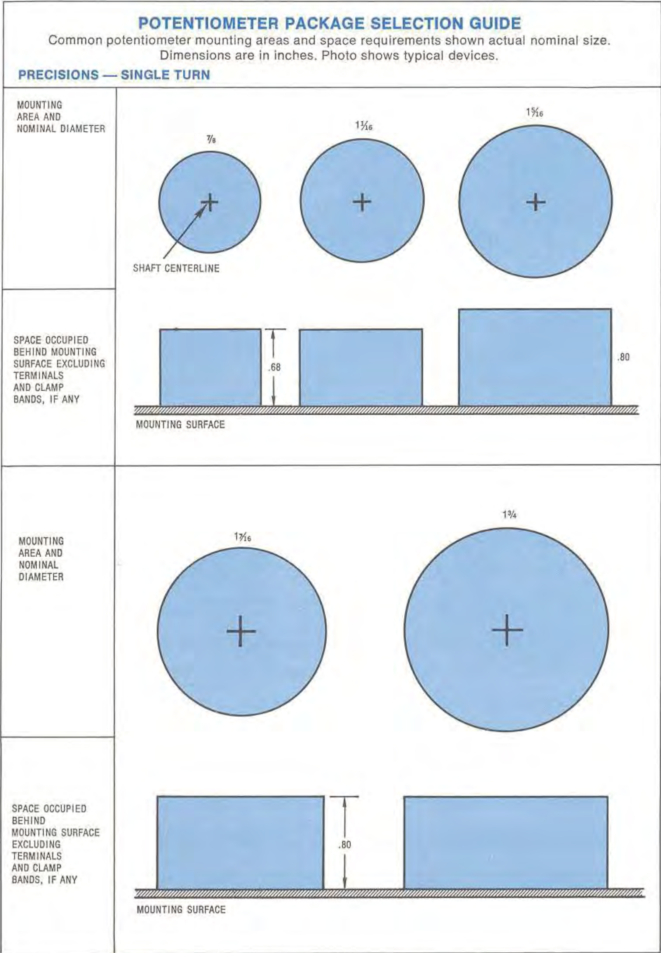
Fig. 8-7 Precision single turn potentiometer package selection guide
