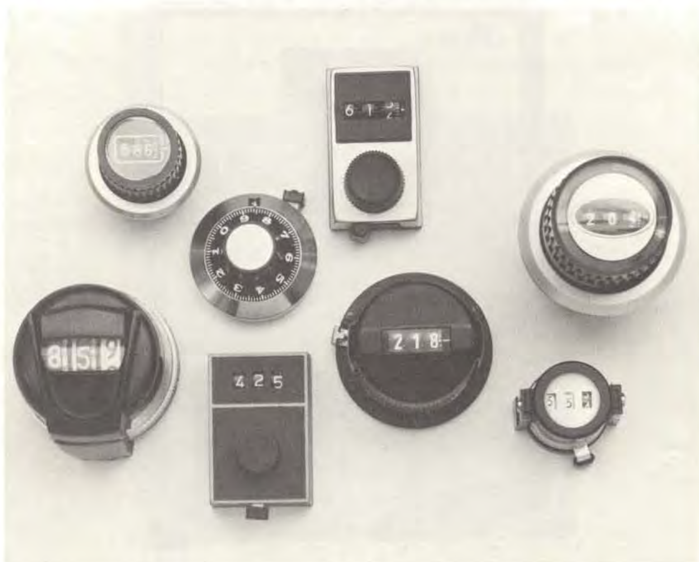
Fig. 3-27 Examples of digital type, multiturn dials
