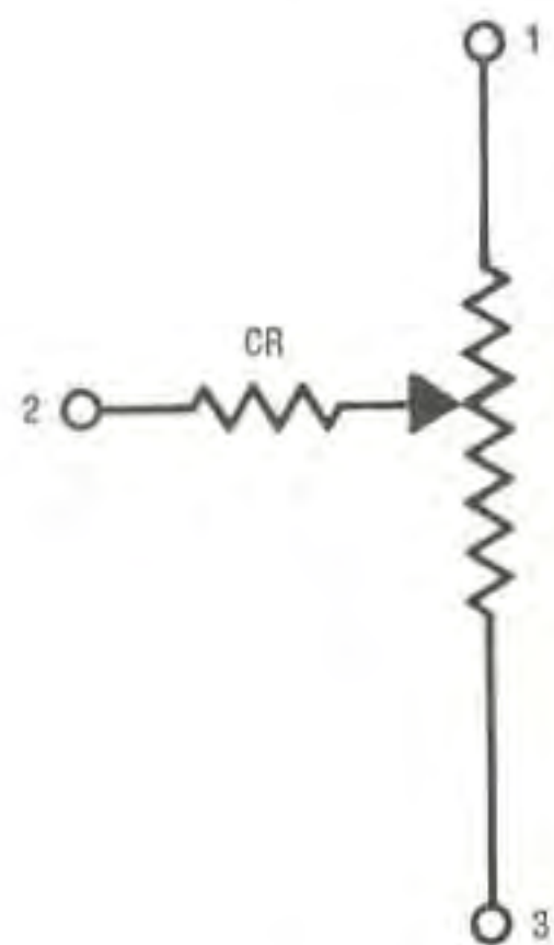
Fig. 2-9 Potentiometer schematic illustrating contact resistance
