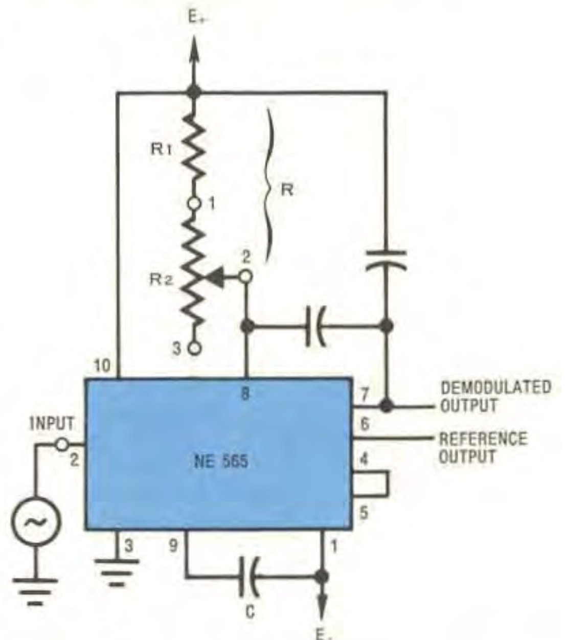
Fig. 4-18 Trimming potentiometers adjusts free-run frequency in a phase locked loop FM demodulator
