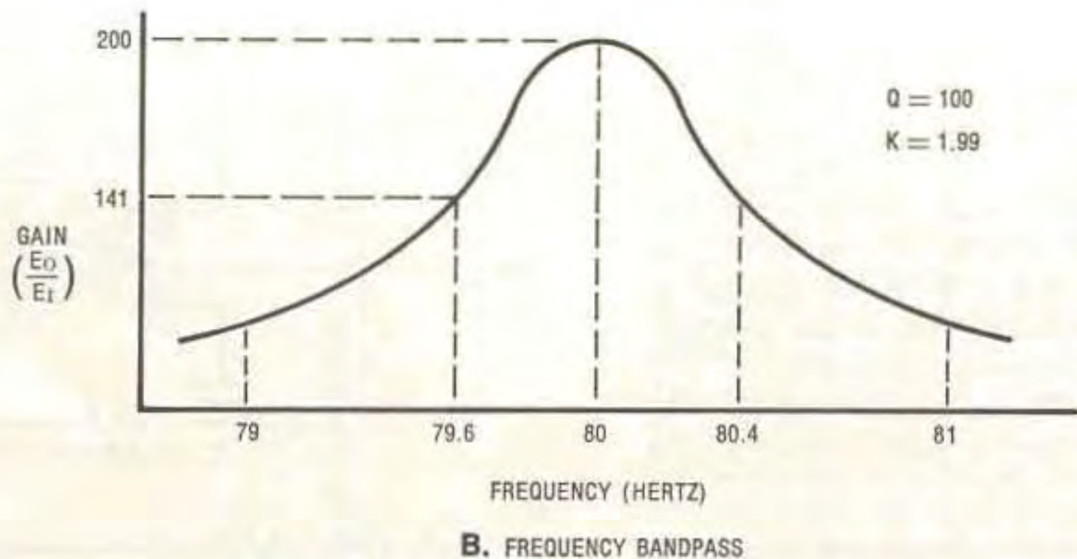
Fig. 4-10 Active band pass filter with variable Q
