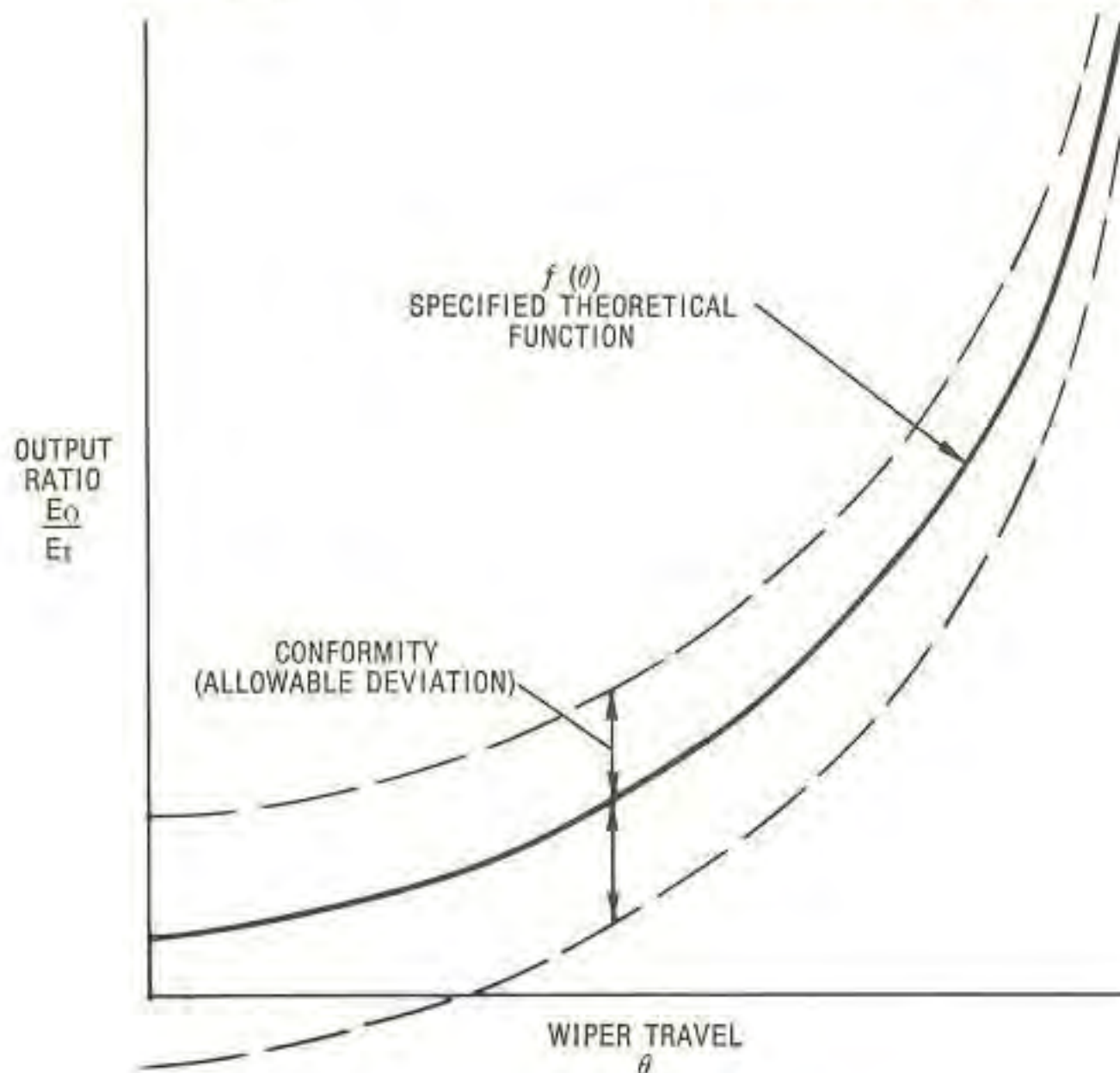
Fig. 2-30 Conformity
