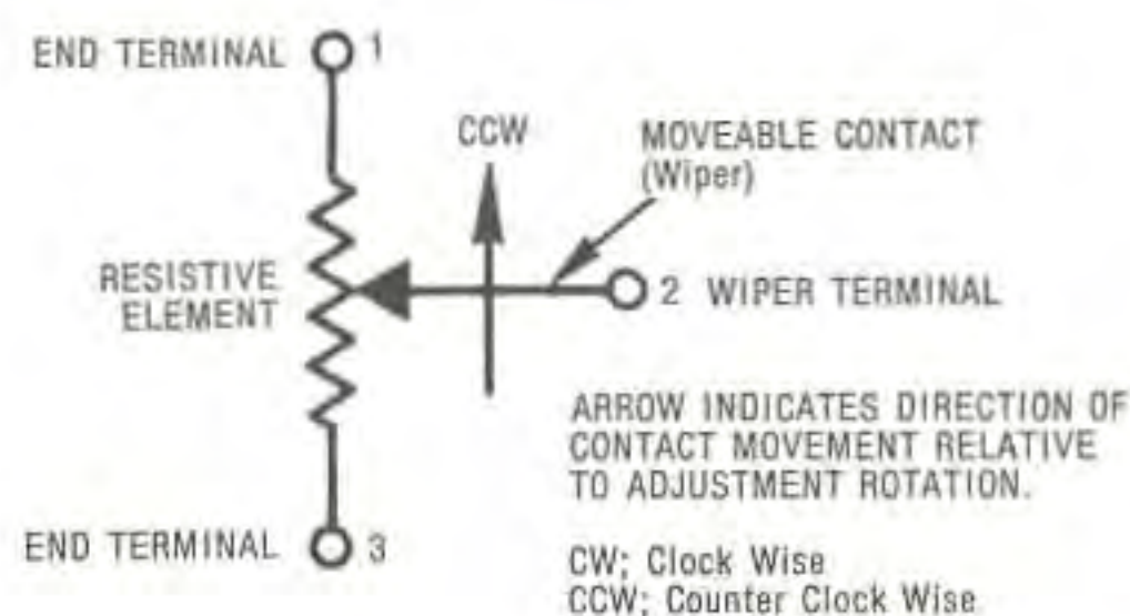
Fig. 2-1 Fundamental schematic representation of variable resistive device
