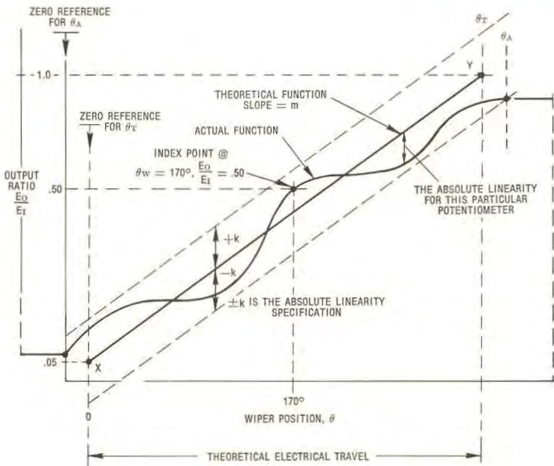
Fig. 2-34 Absolute linearity
