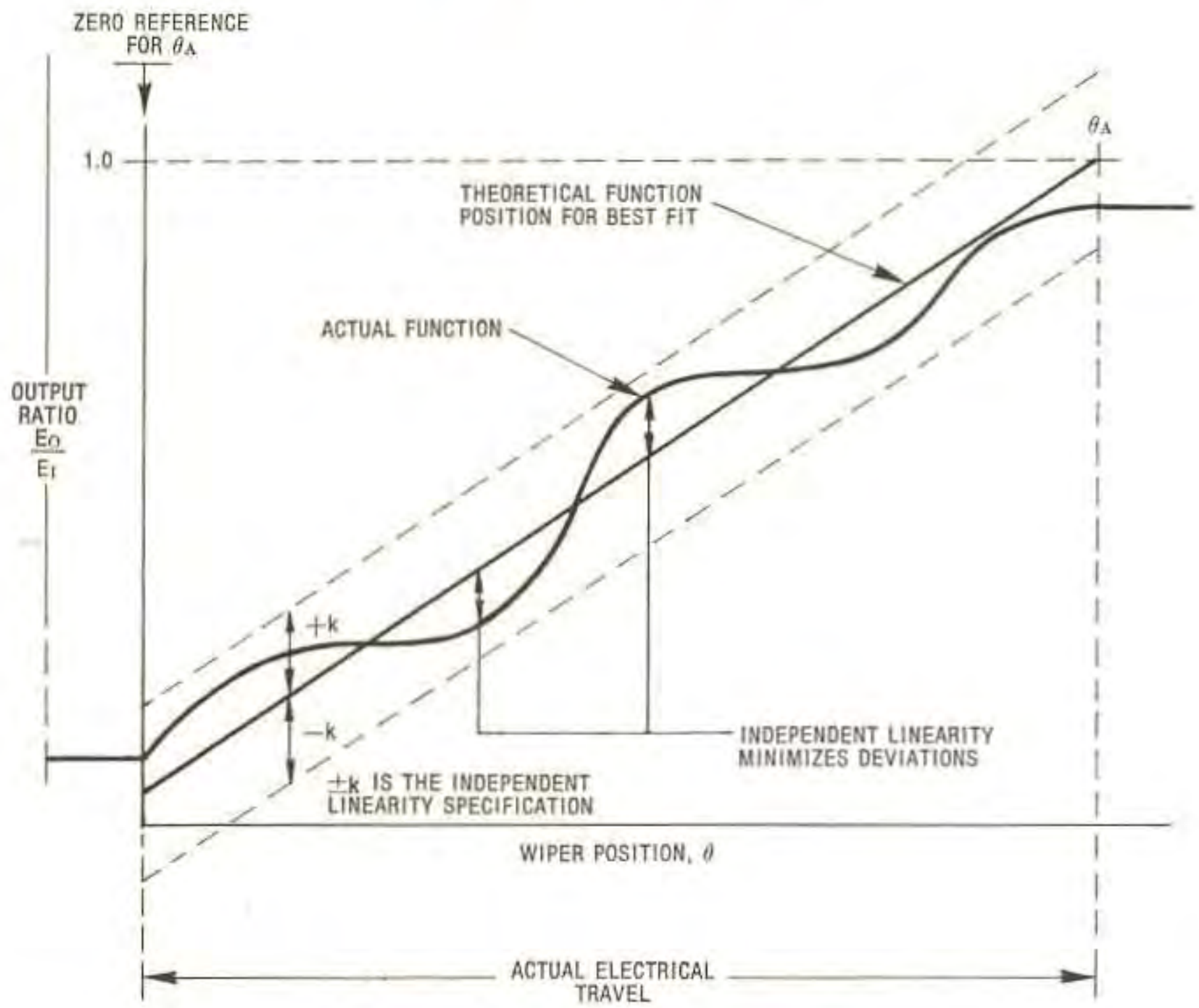
Fig. 2-35 Independent linearity
