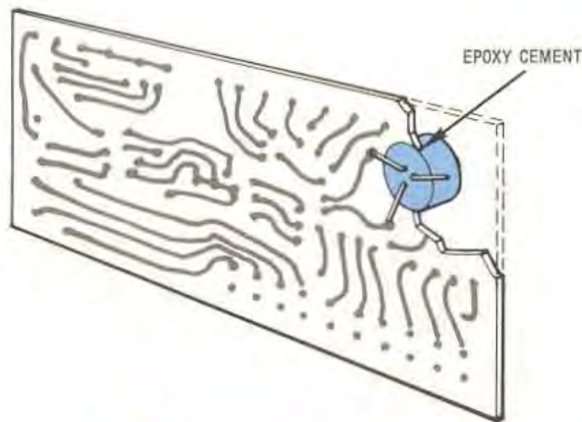
Fig. 8-9 Low-profile mounting
