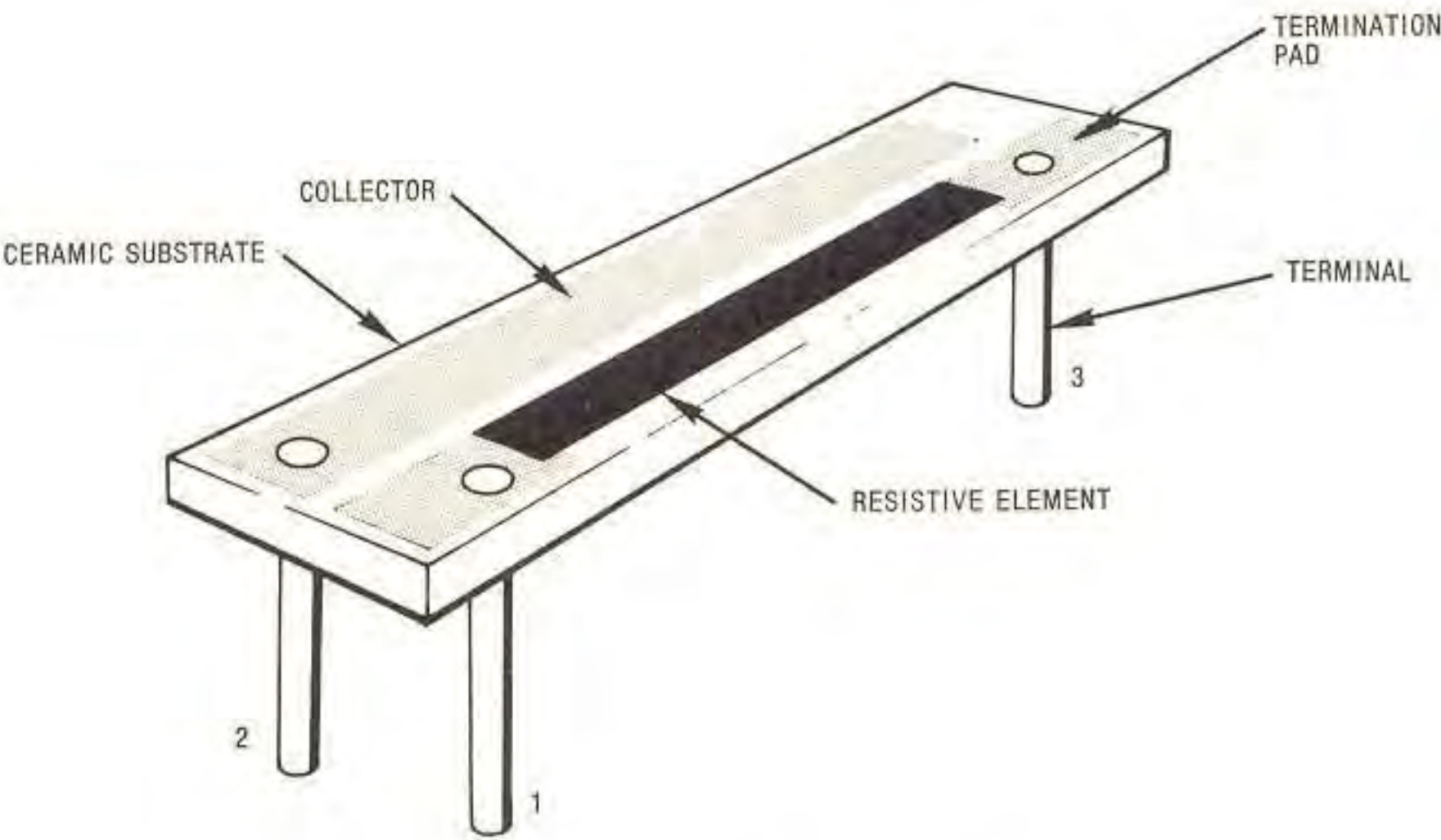
A. A COMMON CERMET POTENTIOMETER CONSTRUCTION
