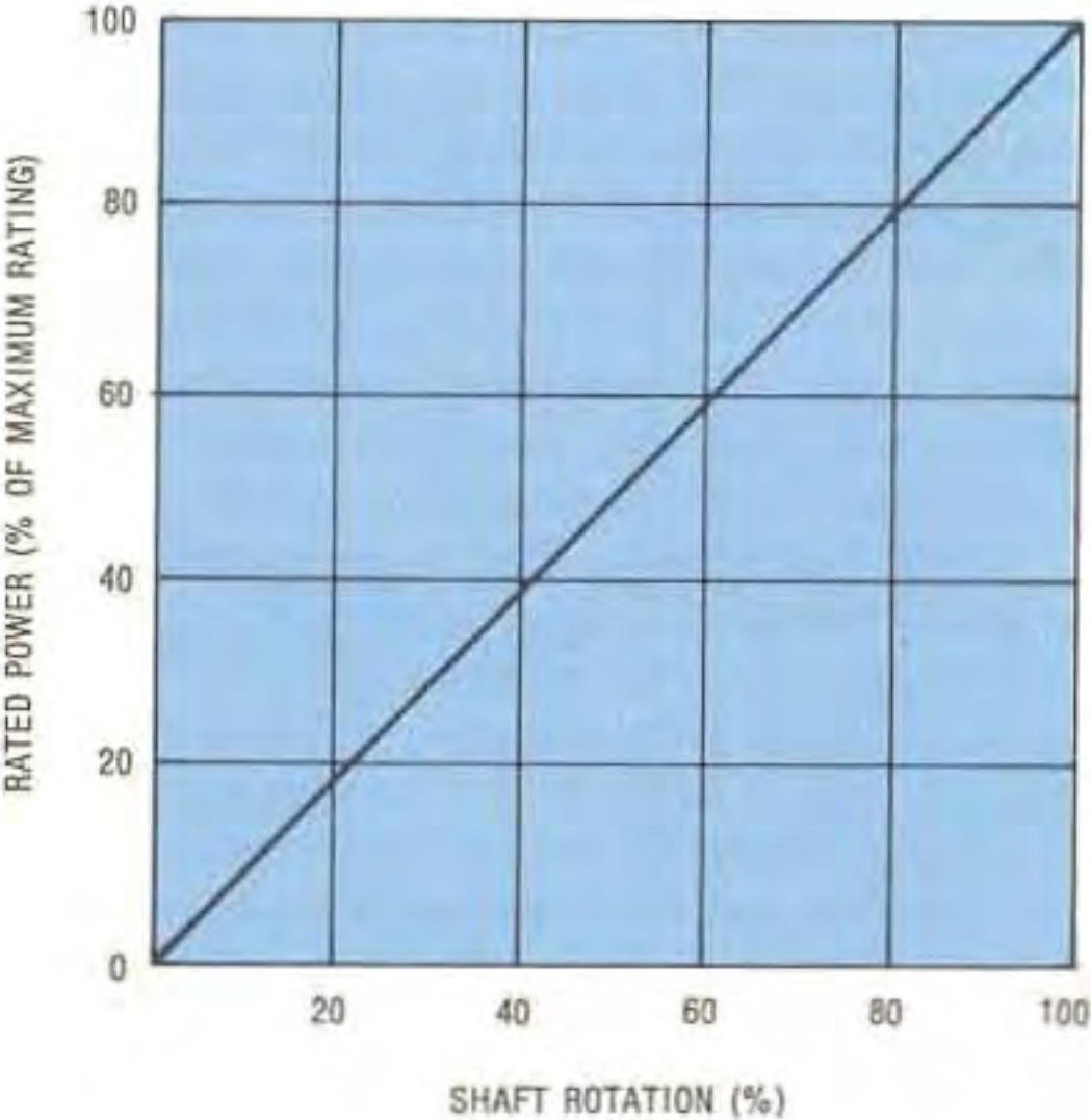
Fig. 6-4 Power derating curve for a rheostat connected, plastic case potentiometer
