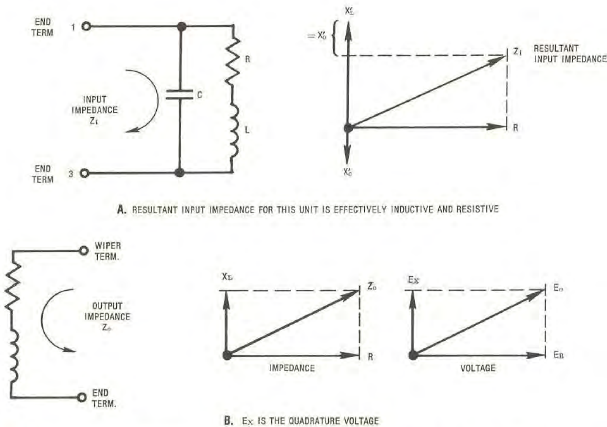
Fig. 6-5 Quadrature voltage for a particular potentiometer at a specified input voltage and frequency
