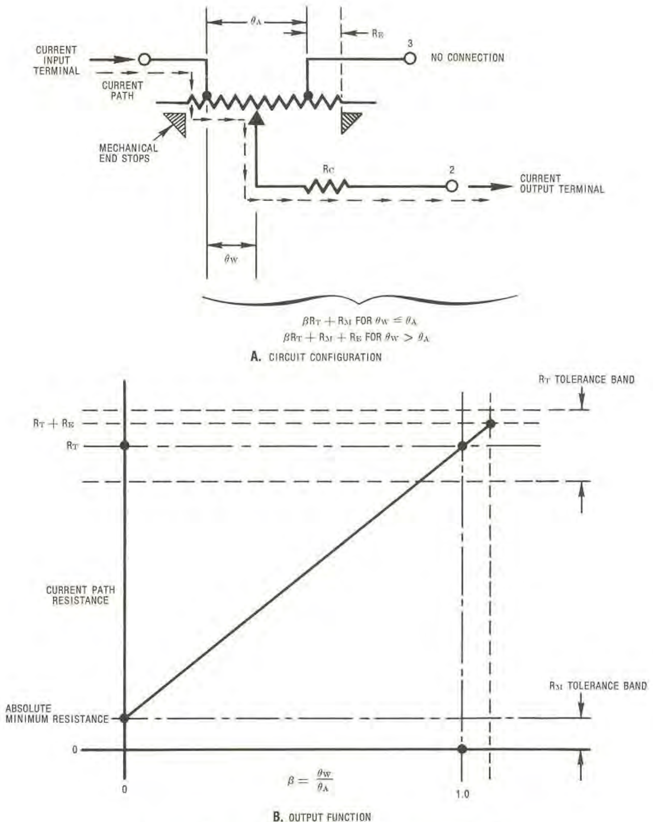
Fig. 3-20 Variable current rheostat mode when R_M \neq R_E
