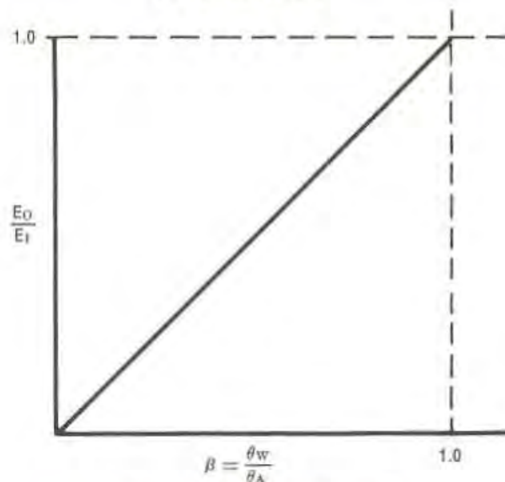
Fig. 3-1 The basic variable voltage divider
