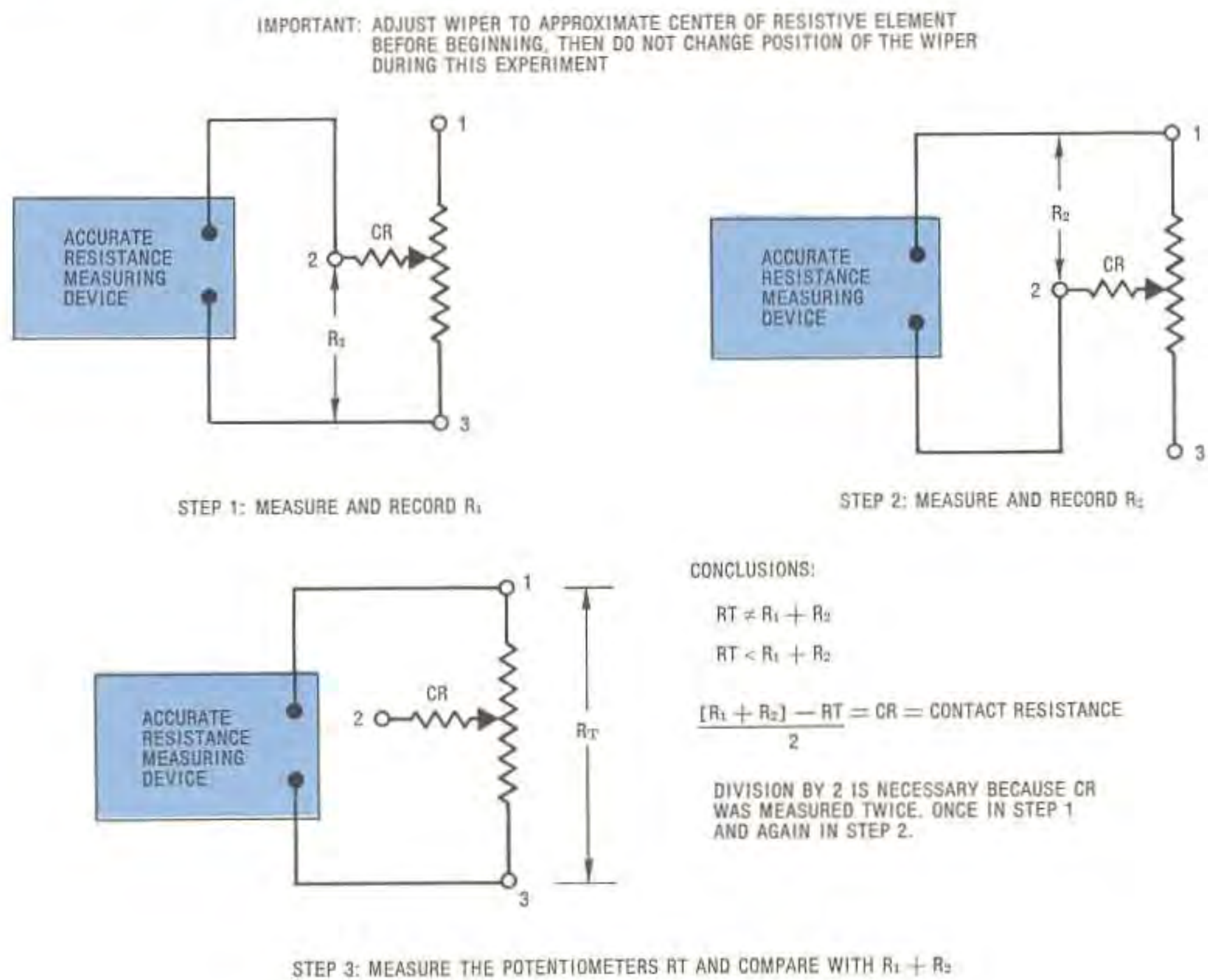
Fig. 2-8 Experiment to demonstrate contact resistance
