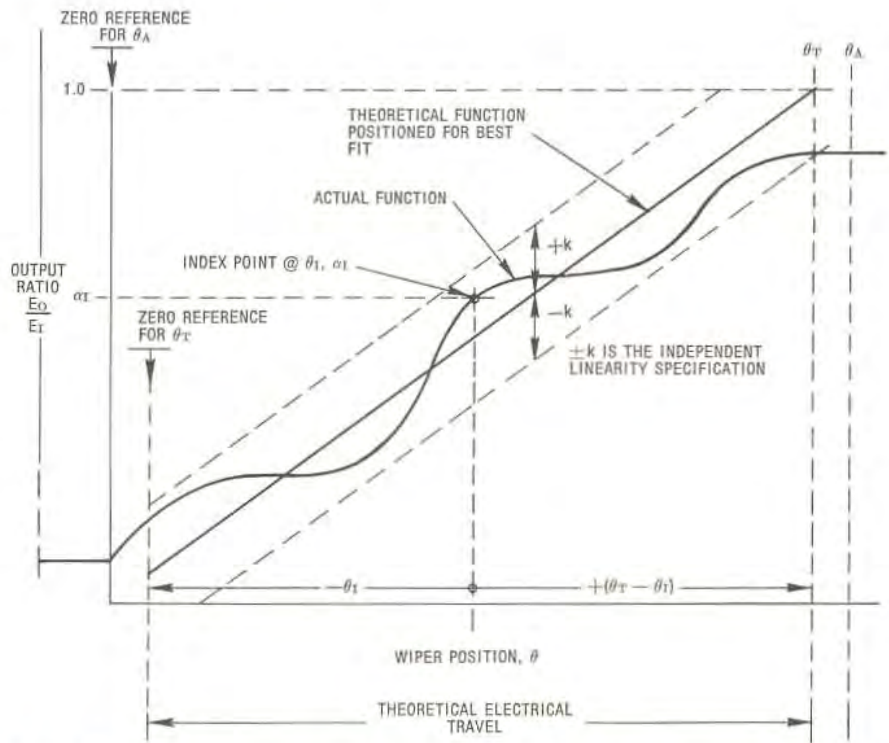
Fig. 2-36 A method to evaluate independent linearity for a non-wirewound potentiometer
