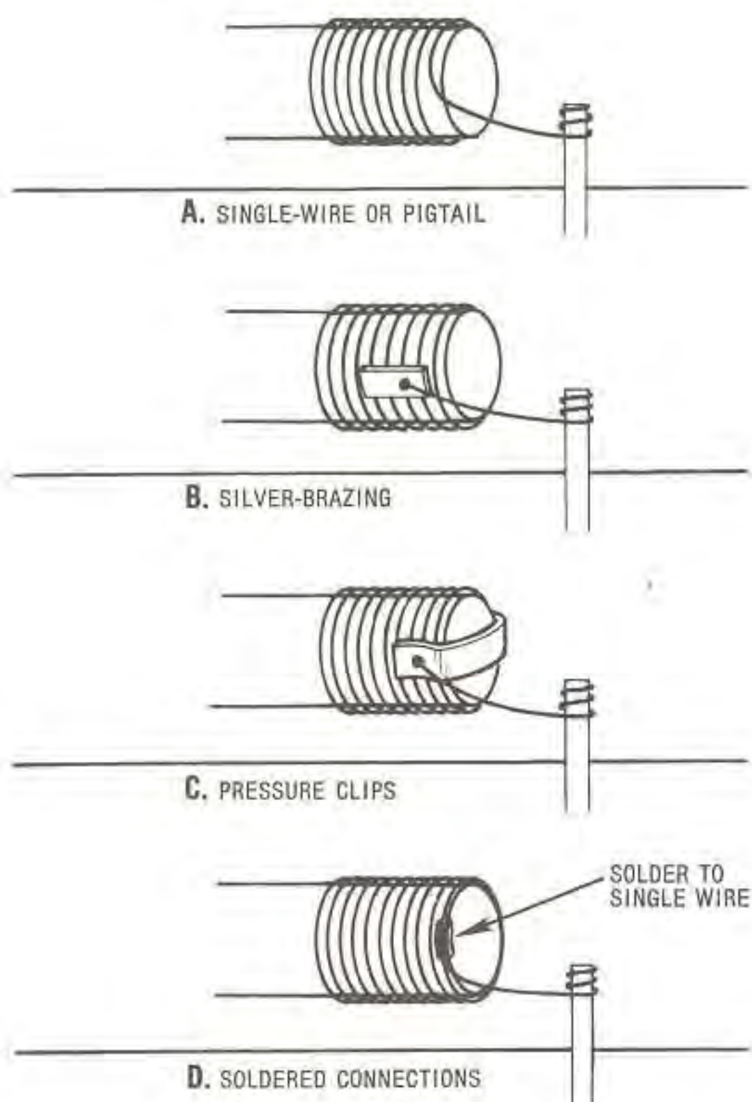
Fig. 7-20 Various methods of element termination for wirewound elements
