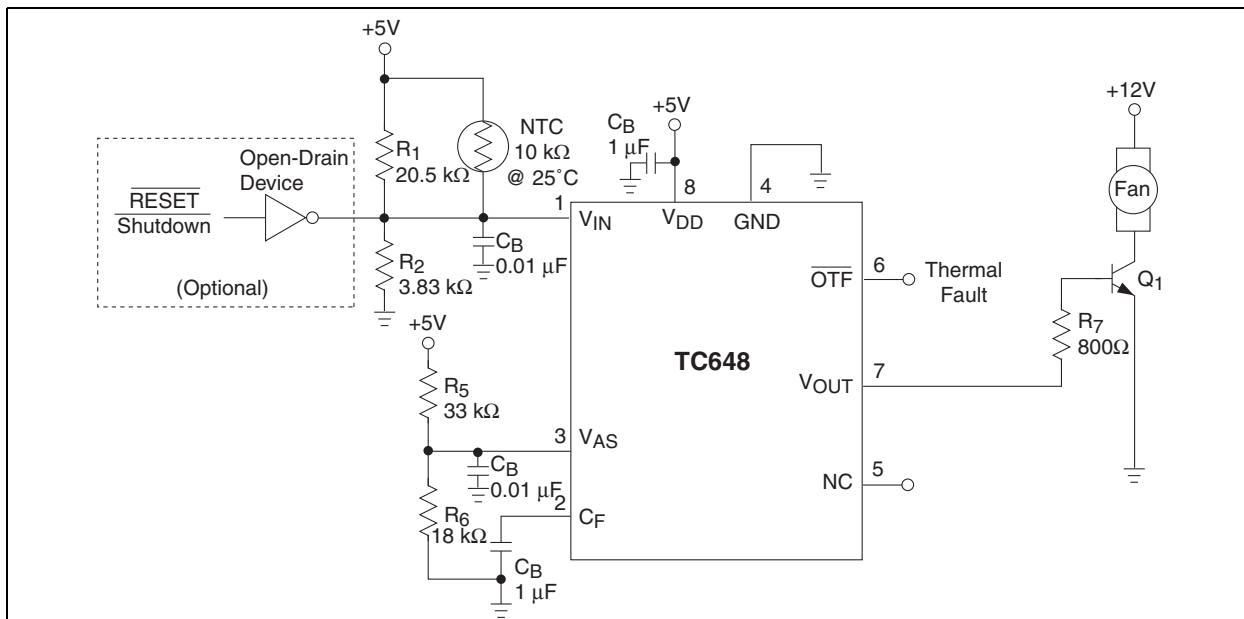
FIGURE 5-8: Design Example.
