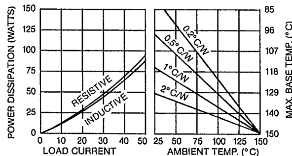
FIGURE 8 — THERMAL DERATING CURVES M5060 (SINGLE PHASE)
