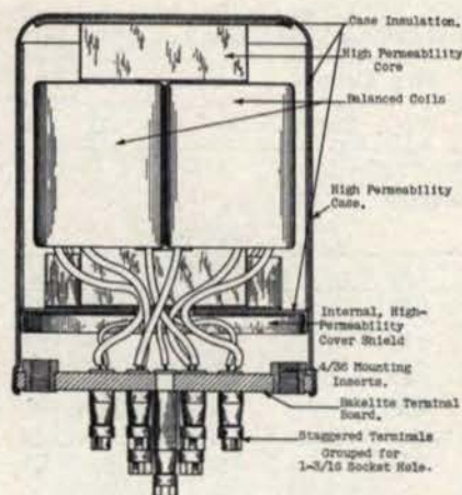
Cross sectional view, Bantam Transformer
