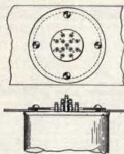
Bottom view, illustrating ring mounting as used in Bantam and Major Series Transformers
