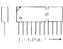
DILP
