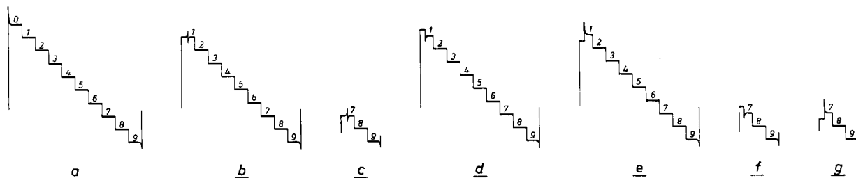
Fig. 30. Oscillograms of a decade incorporating a ten-way switch for the presetting. a — switch at position 0; b — switch at position 1, R_{corr2} accurately adjusted; c — switch at position 7, R_{corr1} accurately adjusted; d — switch at position 1, R_{corr2} too low; e — switch at position 1, R_{corr2} too high; f — switch at position 7, R_{corr1} too high; g — switch at position 7, R_{corr1} too low.
