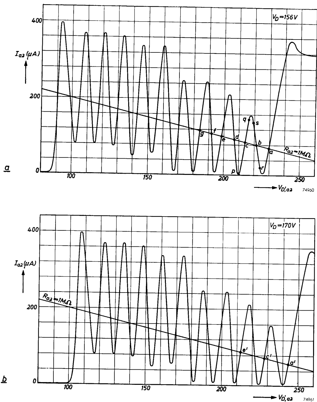
Fig. 6. I_{a2} = f(V_{D',a2}) characteristic for a left deflection electrode voltage V_D = 156 \text{ V} (a) and for V_D = 170 \text{ V} (b).
