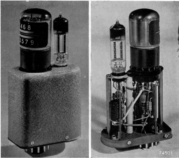
Fig. 16. Interchangeably counter unit comprising an E1T counter tube and an E90CC double triode. The cover of the right-hand unit has been removed to show the accessory components.
