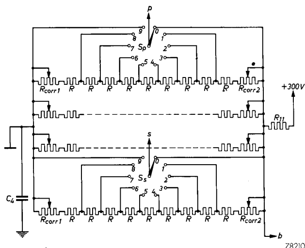
Fig. 25. Circuit for replacing the four wire-wound potentiometers P_1 — P_4 and the resistors R_1 — R_{10} shown in fig. 6 by fixed resistors R ( 4.7 \text{ k}\Omega \pm 2\% , \frac{1}{4} \text{ W} ) and four ten-way switches S_p — S_s . The variable resistors R_{\text{corr}} need be readjusted only when the tubes are replaced. They may be of the carbon type and should have a value of 10 \text{ k}\Omega . Only two of the four branches have been completely drawn. All resistors of this circuit should be mounted such that adequate cooling is provided, this may be done by drilling holes in the chassis above these resistors.
