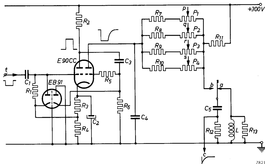
Fig. 24. Circuit of the presetting stage. Point t (input) is connected to the cathode of the last counter tube. The sliders of potentiometers P_1 — P_4 are connected to the cathode of the corresponding diodes incorporated in the individual decades. By pressing the push-button switch at the right, all counter tubes are advanced to position 9; when the switch is subsequently released, so that it returns to position a , the negative-going pulse produced at point c is applied to the input stage, so that all tubes are reset to their predetermined positions.
